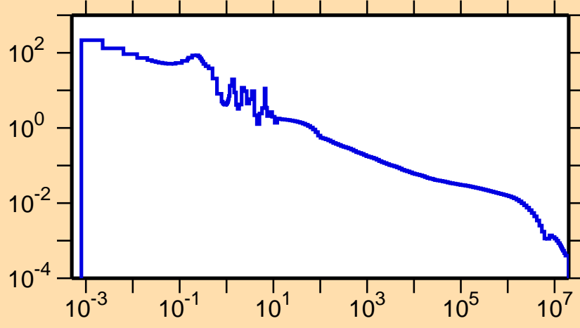
\sigma vs. E for ^{117}\text{Cs}(n,\gamma)
