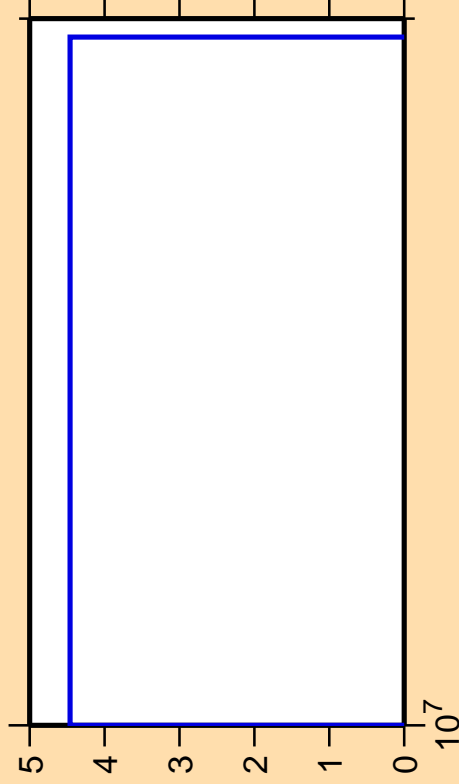
\Delta\sigma/\sigma vs. E for ^{117}\text{Cs}(n,nt)
