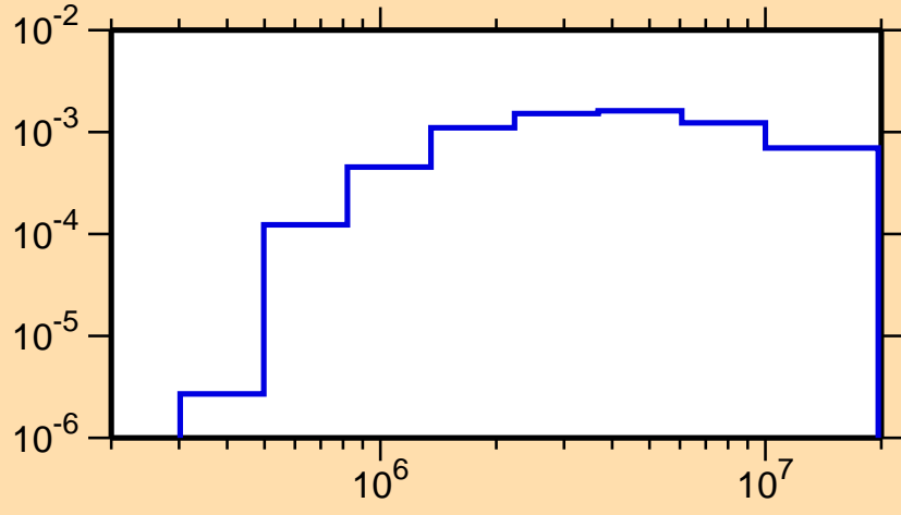
\sigma vs. E for ^{117}\text{Cs}(n,n_3)
