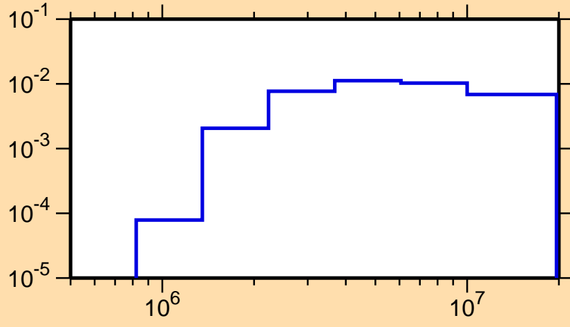
\sigma vs. E for ^{117}\text{Cs}(n,n\text{cont.})
