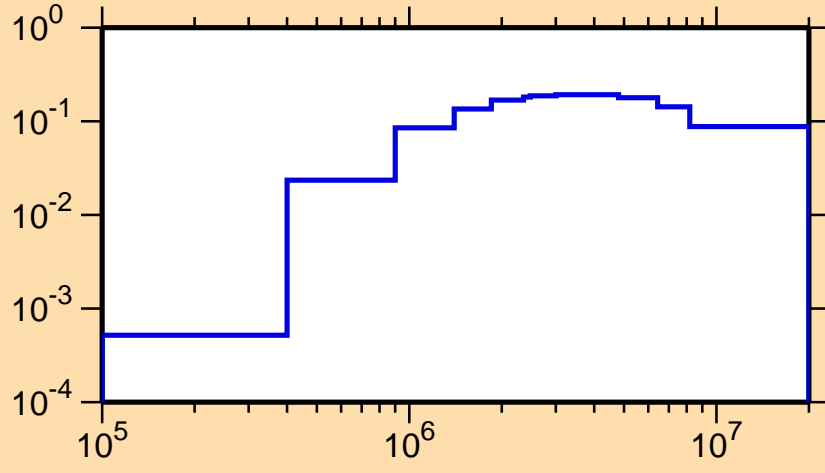
\sigma vs. E for ^{117}\text{Cs}(n,\text{inel.})
