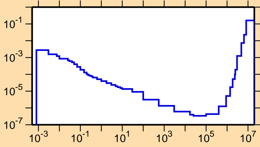
\sigma vs. E for ^{117}\text{Cs}(n,p\alpha)
