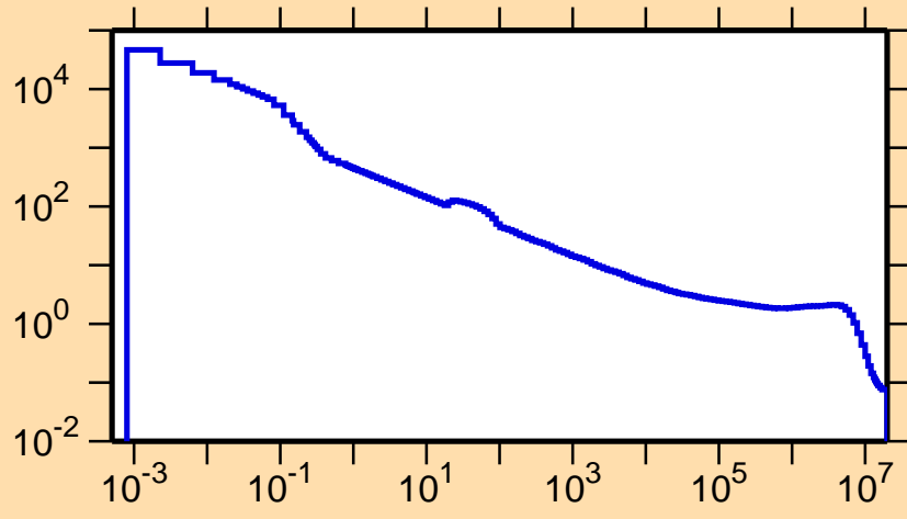
\sigma vs. E for ^{117}\text{Cs}(n,p)
