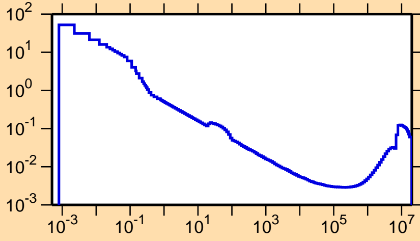
\sigma vs. E for ^{117}\text{Cs}(n,\alpha)
