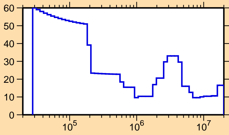
\Delta\sigma/\sigma vs. E for ^{117}\text{Cs}(n, el.)
