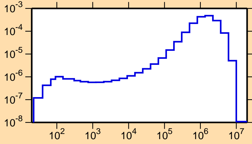
\sigma vs. E for ^{117}\text{Cs}(n,n_2)
