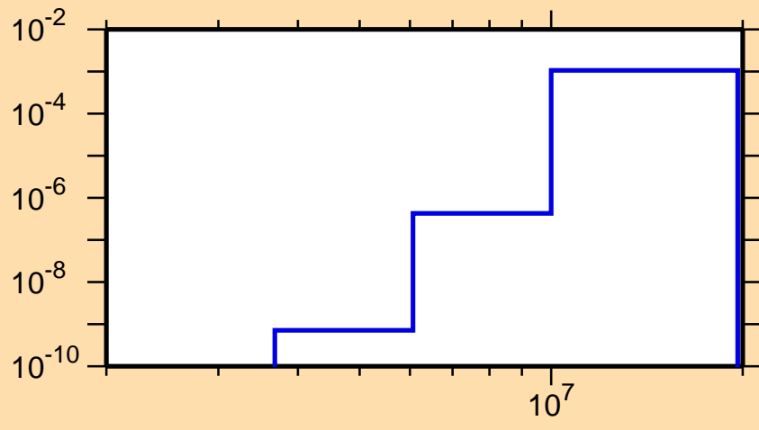
\sigma vs. E for ^{117}\text{Cs}(n,\text{He3})
