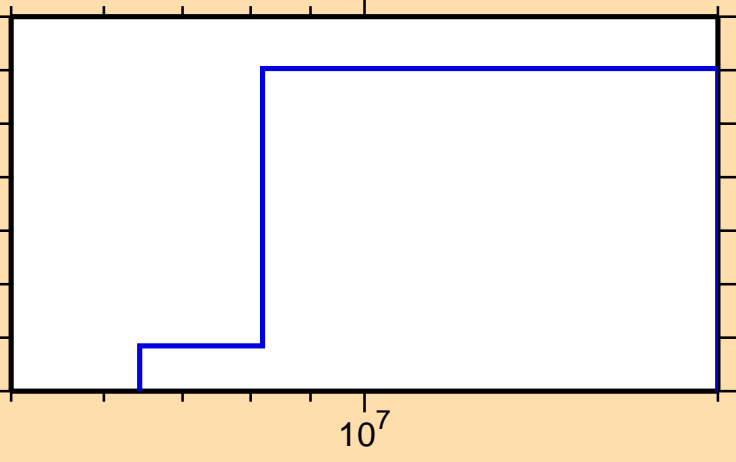
\sigma vs. E for ^{117}\text{Cs}(\text{mt117})
