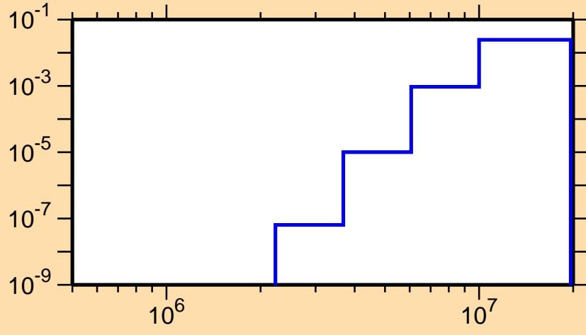
\sigma vs. E for ^{118}\text{Cs}(n,d)
