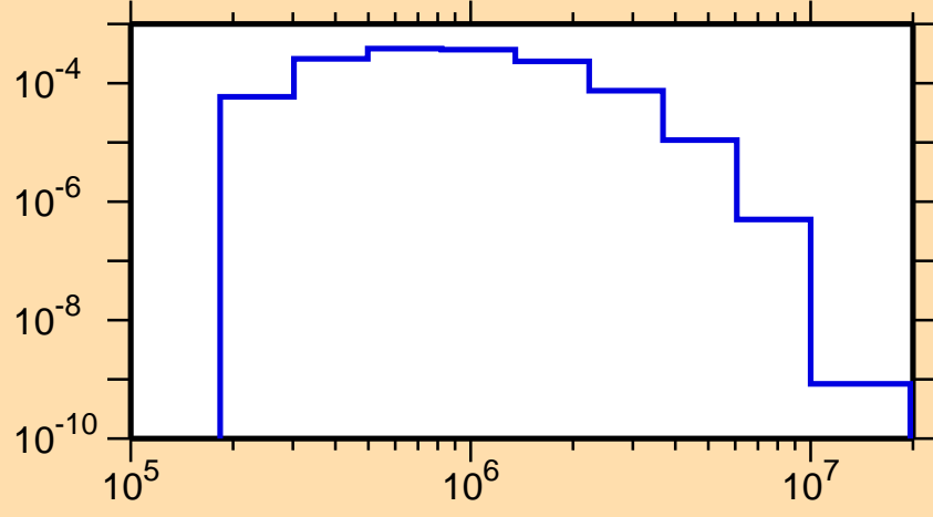
\sigma vs. E for ^{118}\text{Cs}(n,n_1)
