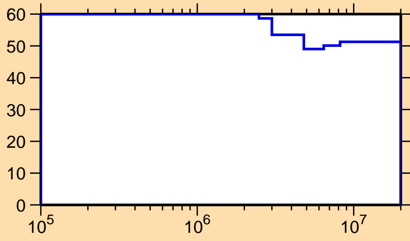
\Delta\sigma/\sigma vs. E for ^{118}\text{Cs}(n,n_1)
