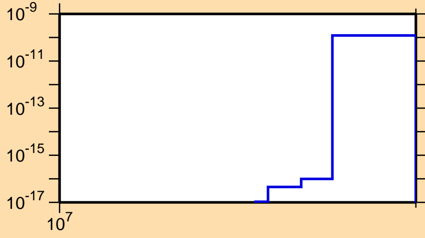
\sigma vs. E for ^{118}\text{Cs}(n,nt)
