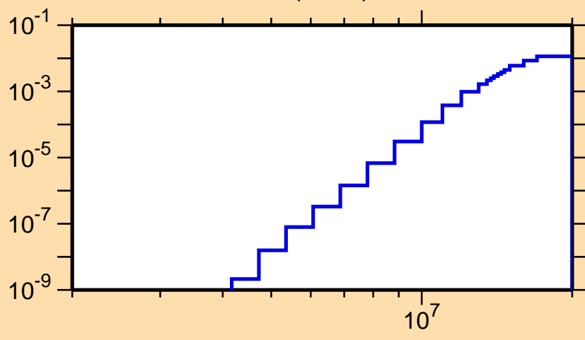
\sigma vs. E for ^{118}\text{Cs}(n,n\alpha)
