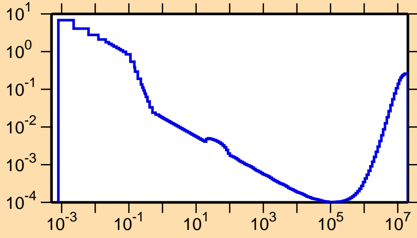
\sigma vs. E for ^{118}\text{Cs}(n,p\alpha)
