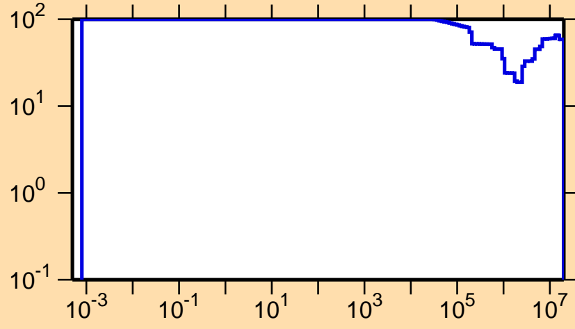
\Delta\sigma/\sigma vs. E for ^{118}\text{Cs}(n,p)
