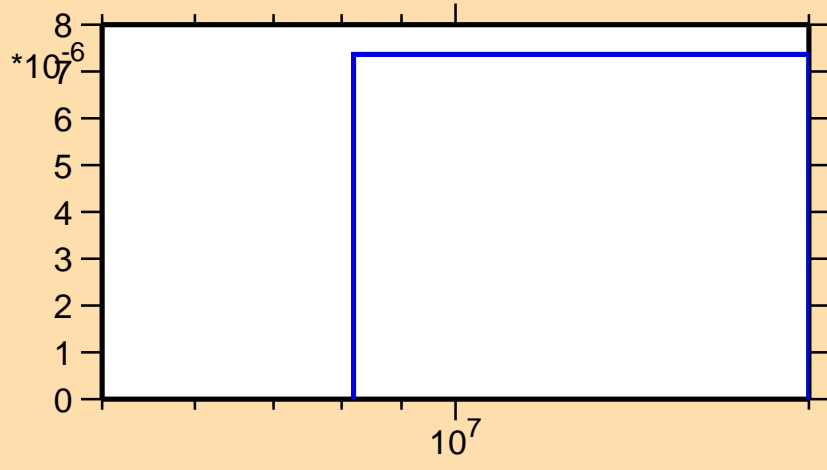
\sigma vs. E for ^{118}\text{Cs}(n,nd)
