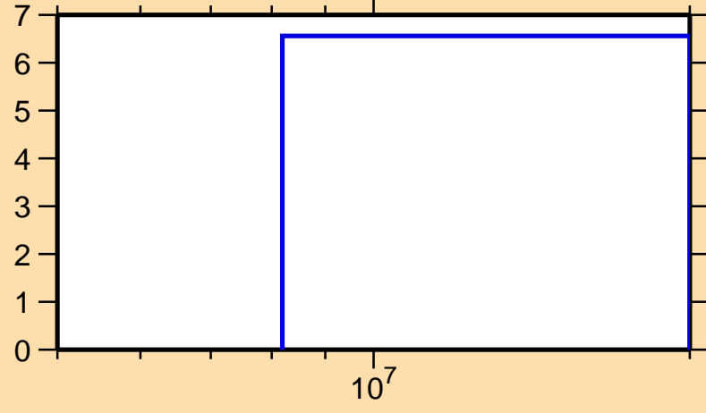
\Delta\sigma/\sigma vs. E for ^{118}\text{Cs}(n,\text{el.})
