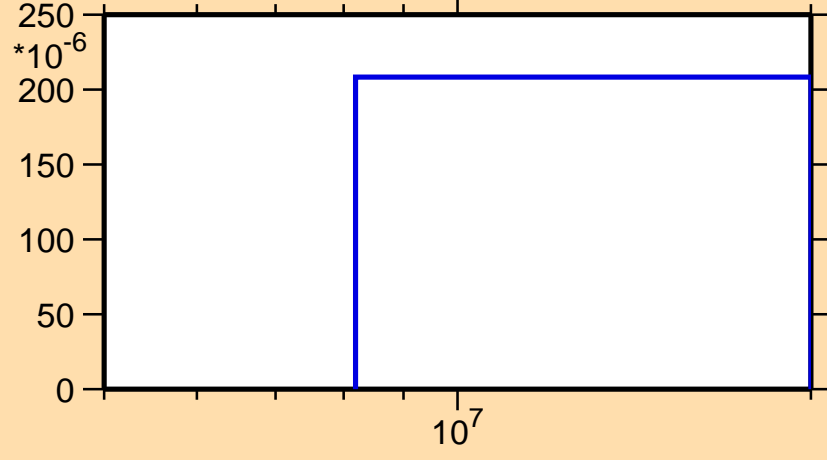
\sigma vs. E for ^{118}\text{Cs}(n,2np)
