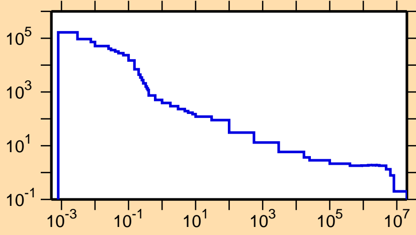
\sigma vs. E for ^{118}\text{Cs}(n,p)
