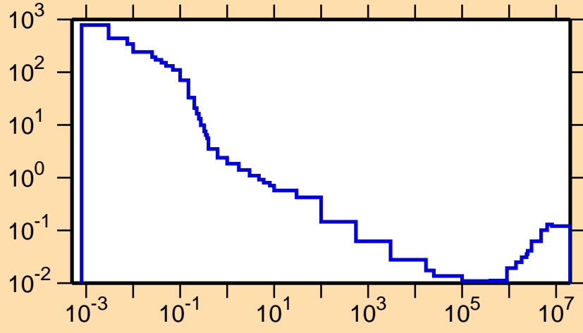
\sigma vs. E for ^{118}\text{Cs}(n,\alpha)
