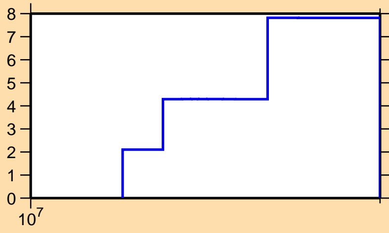
\Delta\sigma/\sigma vs. E for ^{119}\text{Cs}(n,\text{tot.})
