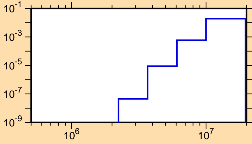
\sigma vs. E for ^{119}\text{Cs}(n,d)
