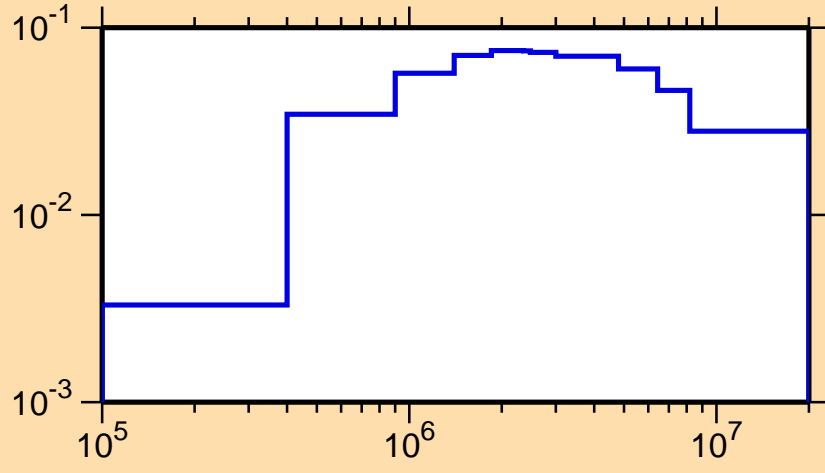
\sigma vs. E for ^{119}\text{Cs}(n,n_2)
