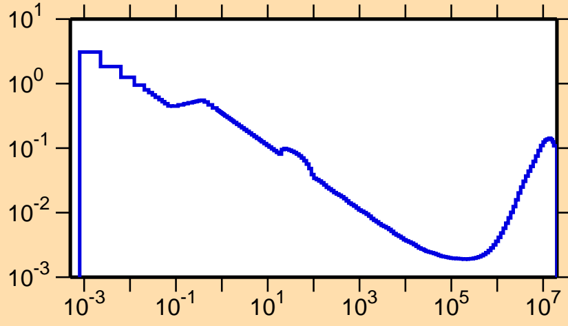
\sigma vs. E for ^{119}\text{Cs}(n,\alpha)
