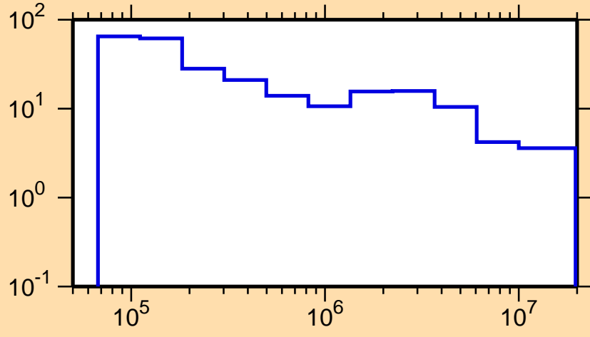
\Delta\sigma/\sigma vs. E for ^{119}\text{Cs}(n, tot.)
