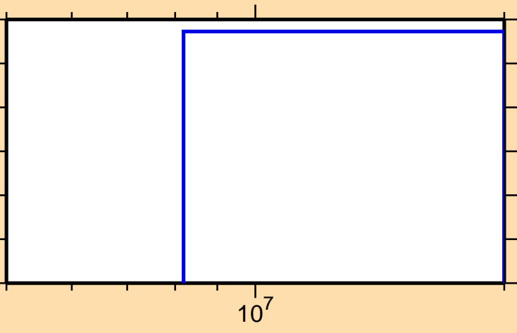
\sigma vs. E for ^{119}\text{Cs}(n,2np)
