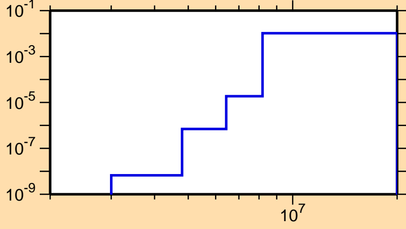
\sigma vs. E for ^{119}\text{Cs}(n,n\alpha)
