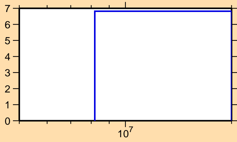
\Delta\sigma/\sigma vs. E for ^{119}\text{Cs}(n,\text{el.})
