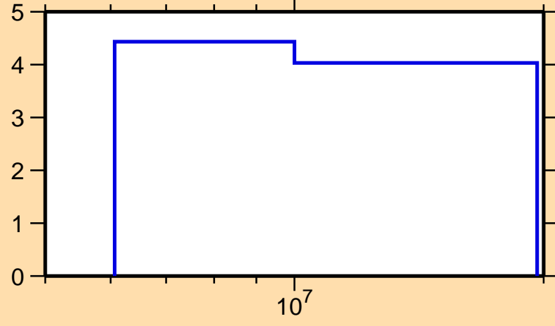
\Delta\sigma/\sigma vs. E for ^{120}\text{Cs}(n,\text{tot.})
