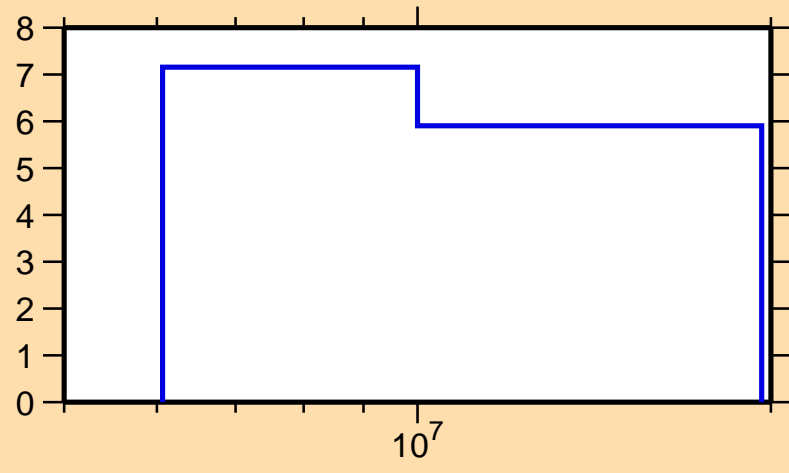
\Delta\sigma/\sigma vs. E for ^{120}\text{Cs}(n,\text{nonel.})
