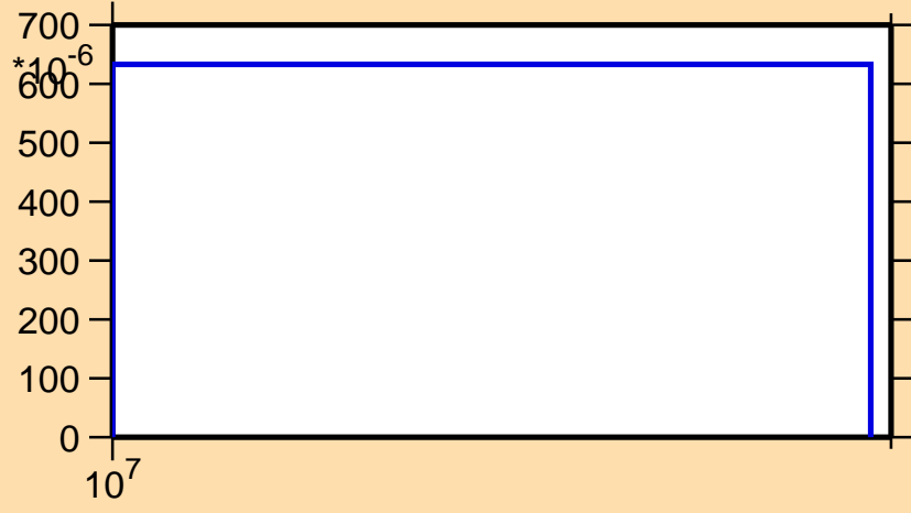
\sigma vs. E for ^{120}\text{Cs}(n,2np)
