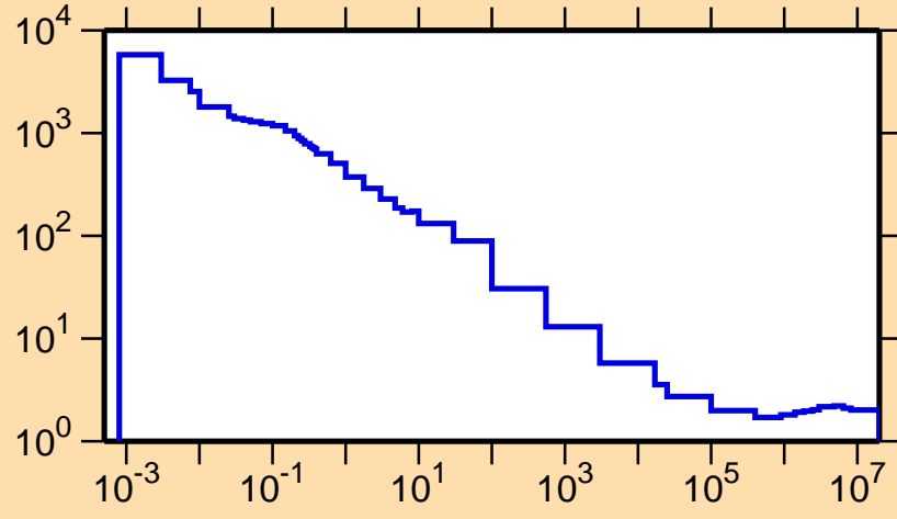
\sigma vs. E for ^{120}\text{Cs}(n,\text{nonel.})
