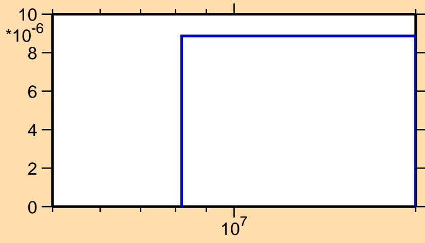
\sigma vs. E for ^{120}\text{Cs}(n,\text{nd})
