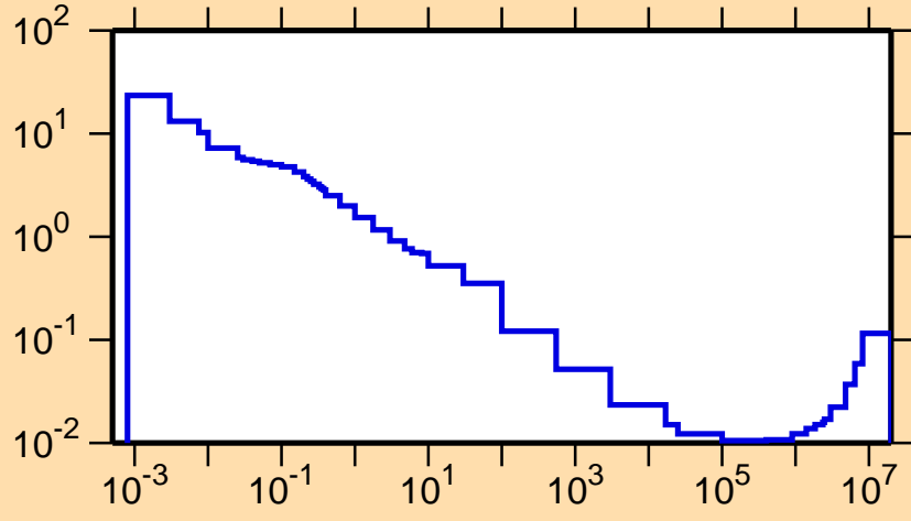
\sigma vs. E for ^{120}\text{Cs}(n,\alpha)
