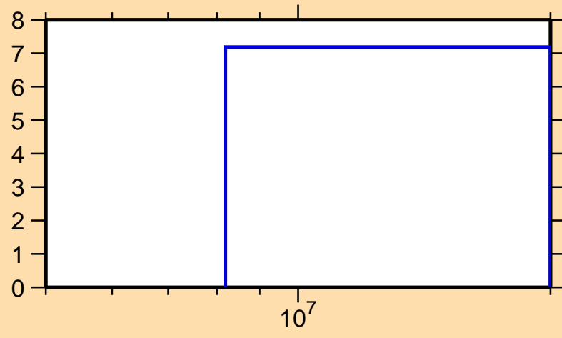
\Delta\sigma/\sigma vs. E for ^{120}\text{Cs}(n,\text{el.})
