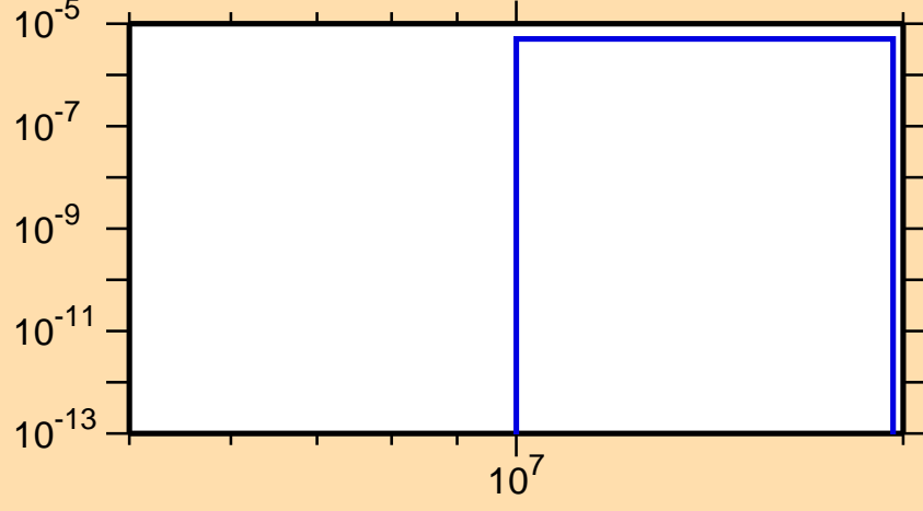
\sigma vs. E for ^{120}\text{Cs} (mt 45)
