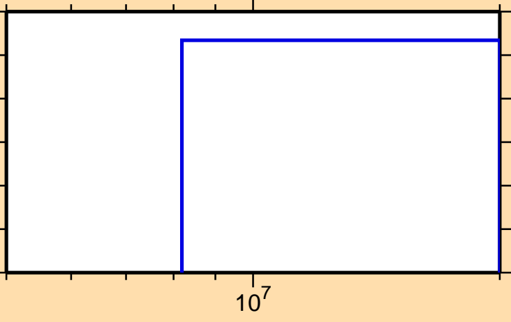
\sigma vs. E for ^{120}\text{Cs}(\text{mt117})
