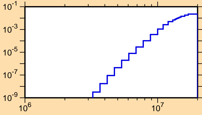
\sigma vs. E for ^{121}\text{Cs}(n,p\alpha)
