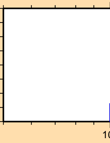
\sigma vs. E for ^{121}\text{Cs}(\text{mt117})
