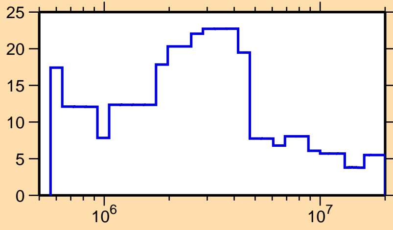
\Delta\sigma/\sigma vs. E for ^{121}\text{Cs}(n, el.)
