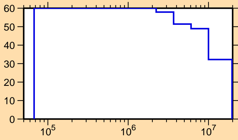
\Delta\sigma/\sigma vs. E for ^{121}\text{Cs}(n,n_1)
