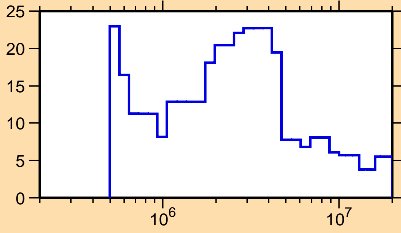
\Delta\sigma/\sigma vs. E for ^{121}\text{Cs}(n, el.)
