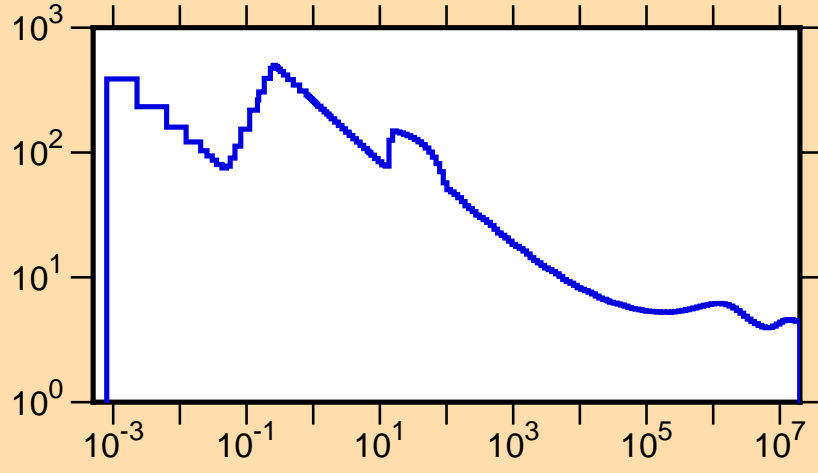
\sigma vs. E for ^{121}\text{Cs}(n,\text{tot.})
