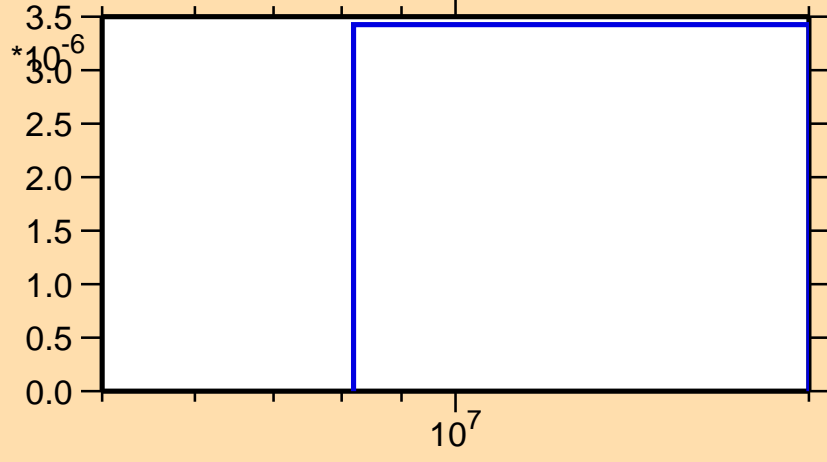
\sigma vs. E for ^{121}\text{Cs} (mt 45)
