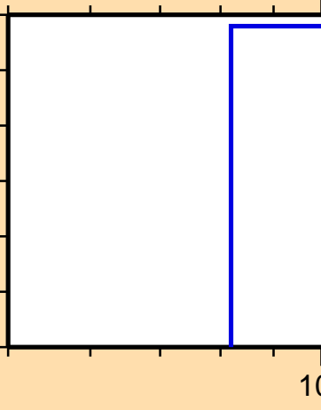
\sigma vs. E for ^{121}\text{Cs}(n,pt)
