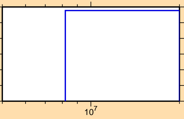
\sigma vs. E for ^{121}\text{Cs}(n,2np)
