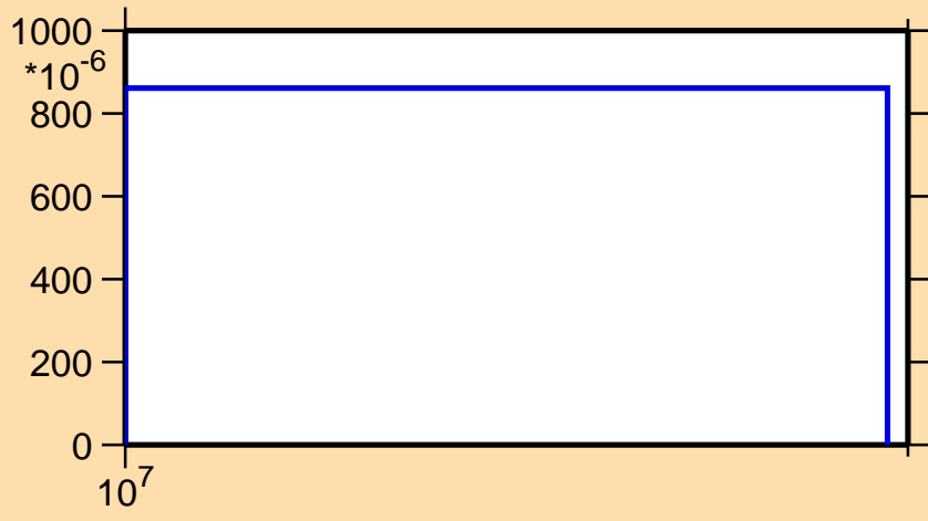
\sigma vs. E for ^{122}\text{Cs}(n,2np)
