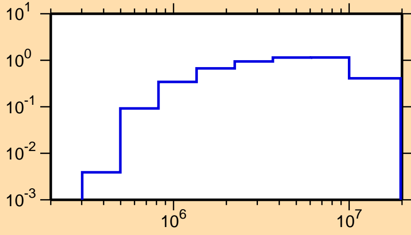
\sigma vs. E for ^{122}\text{Cs}(n,n\text{cont.})
