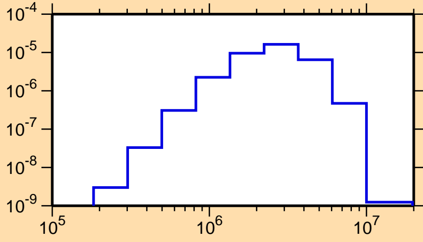
\sigma vs. E for ^{122}\text{Cs}(n,n_1)
