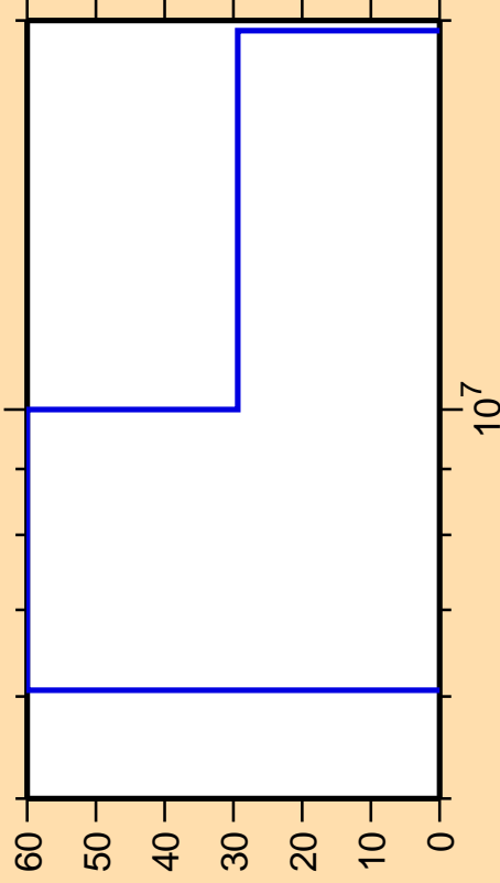
\Delta\sigma/\sigma vs. E for ^{122}\text{Cs}(n,2n)
