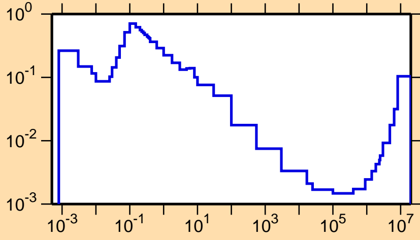
\sigma vs. E for ^{122}\text{Cs}(n,\alpha)
