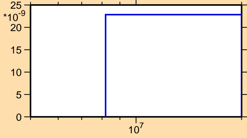
\sigma vs. E for ^{122}\text{Cs}(n,2n\alpha)
