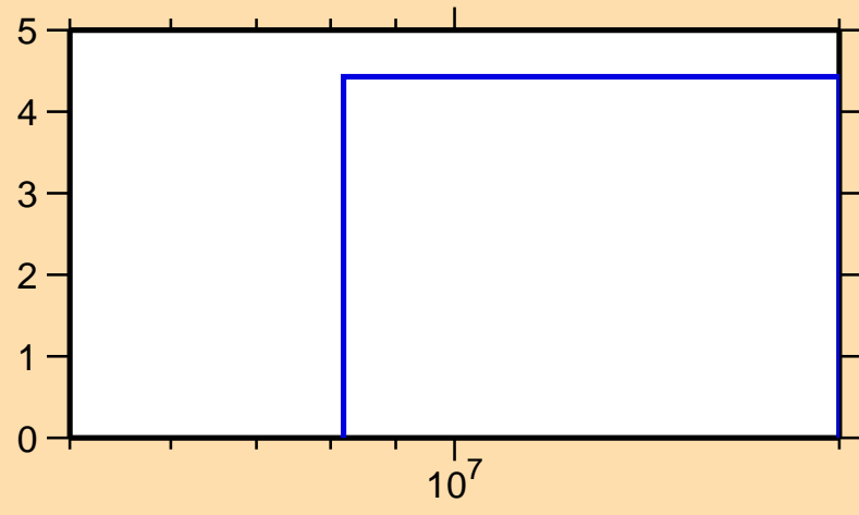
\Delta\sigma/\sigma vs. E for ^{122}\text{Cs}(n,\text{tot.})
