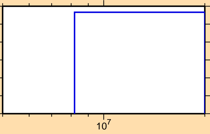
\sigma vs. E for ^{122}\text{Cs}(n,\text{pd})
