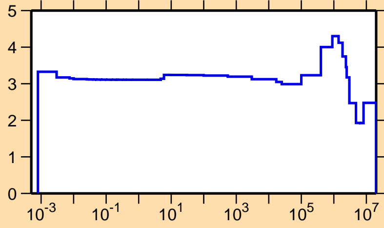
\sigma vs. E for ^{122}\text{Cs}(n,\text{el.})
