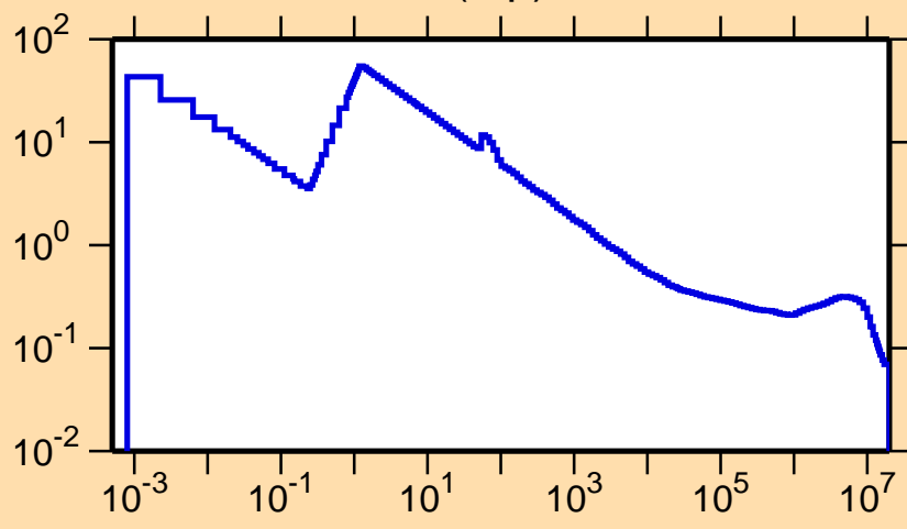
\sigma vs. E for ^{123}\text{Cs}(n,p)
