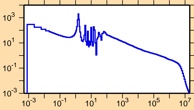
\sigma vs. E for ^{123}\text{Cs}(n,\gamma)
