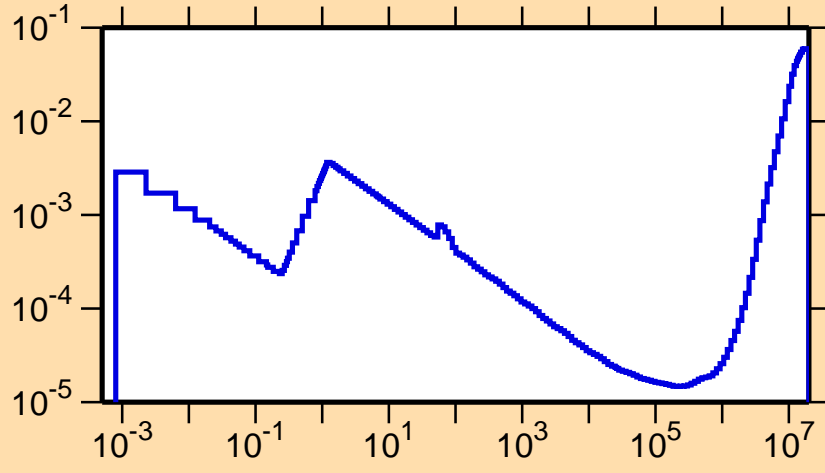
\sigma vs. E for ^{123}\text{Cs}(n,\alpha)
