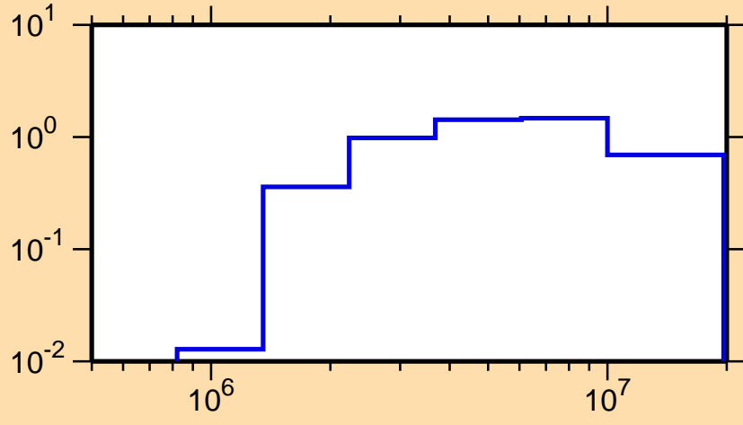
\sigma vs. E for ^{123}\text{Cs}(n,n\text{cont.})
