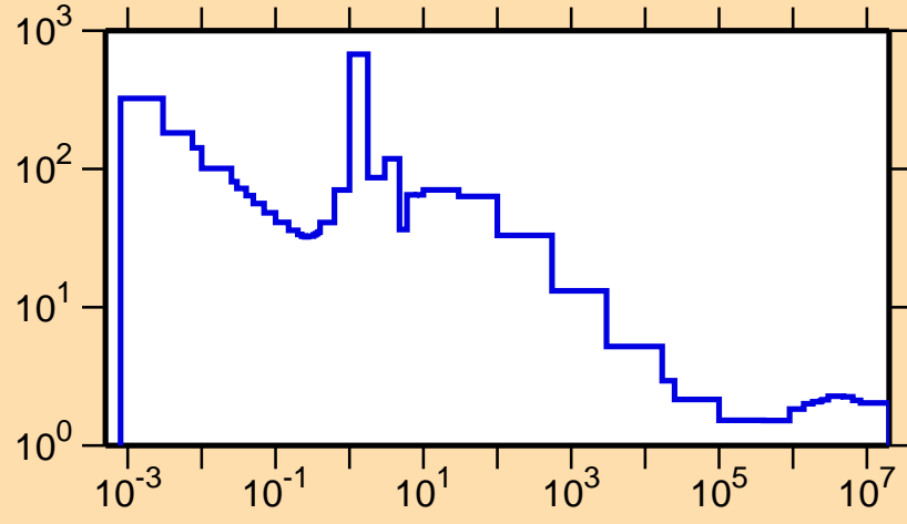
\sigma vs. E for ^{123}\text{Cs}(n,\text{nonel.})
