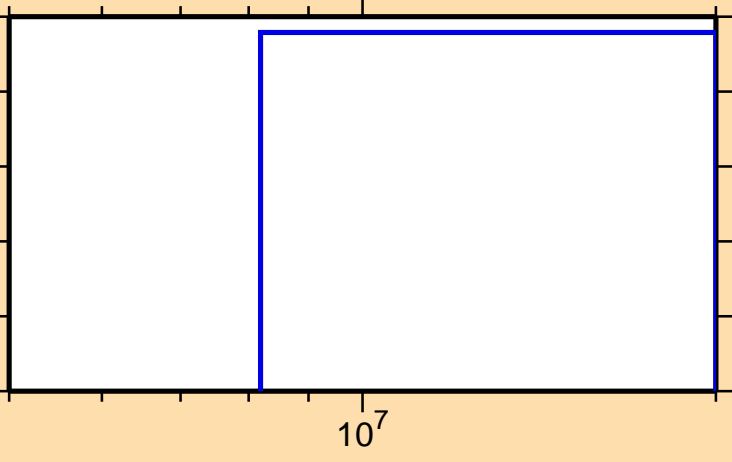
\sigma vs. E for ^{123}\text{Cs} (mt 45)
