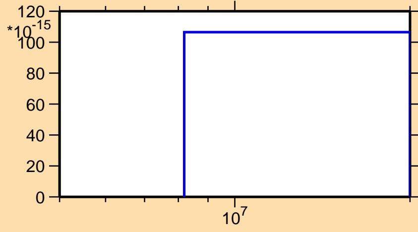
\sigma vs. E for ^{123}\text{Cs}(n,pt)
