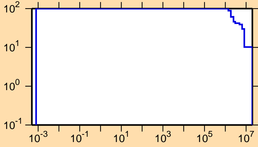
\Delta\sigma/\sigma vs. E for ^{123}\text{Cs}(n,p)
