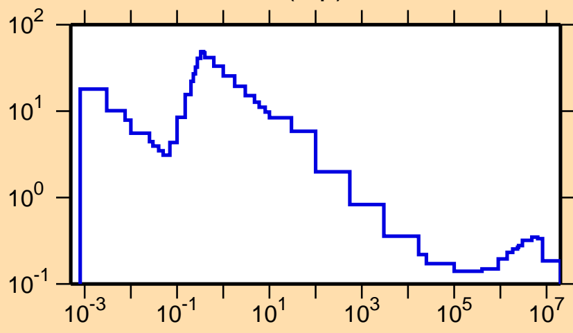
\sigma vs. E for ^{123}\text{Cs}(n,p)
