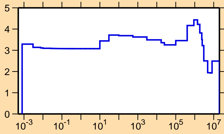
\sigma vs. E for ^{123}\text{Cs}(n,\text{el.})
