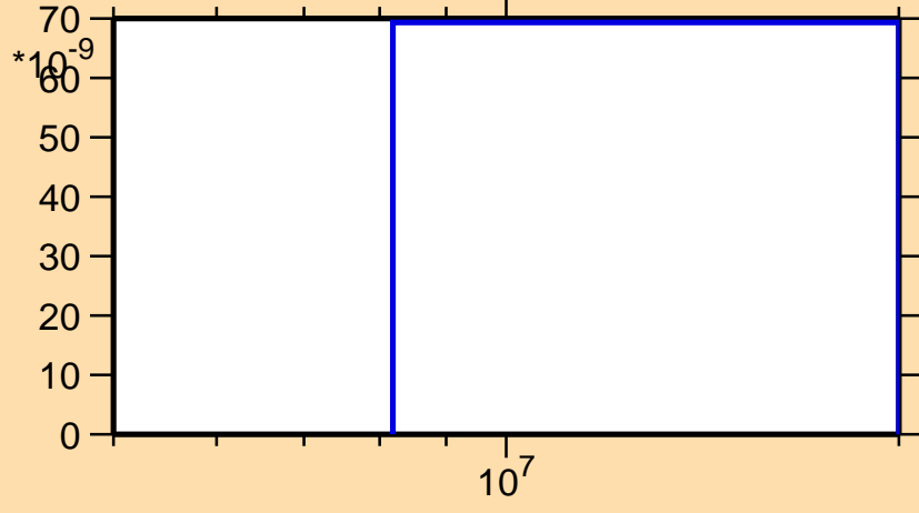
\sigma vs. E for ^{123}\text{Cs} (mt 45)
