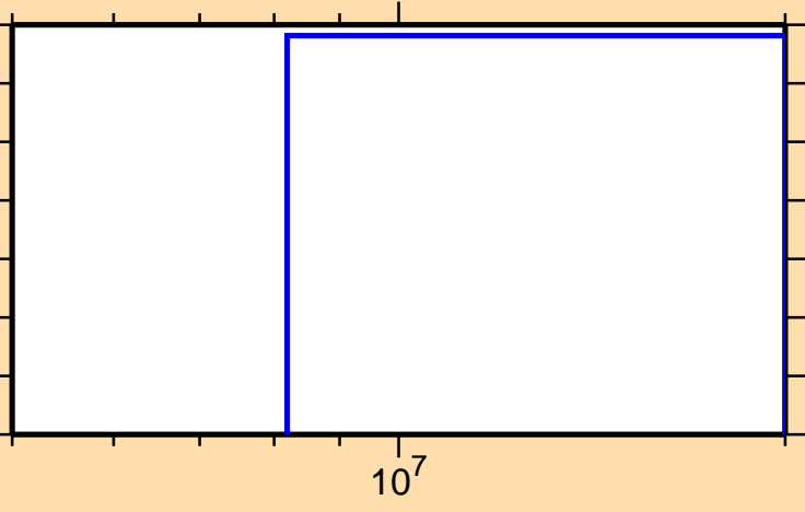
\sigma vs. E for ^{123}\text{Cs}(n,2n)
