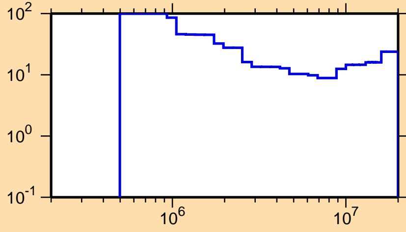
\Delta\sigma/\sigma vs. E for ^{124}\text{Cs}(n,n\text{cont.})
