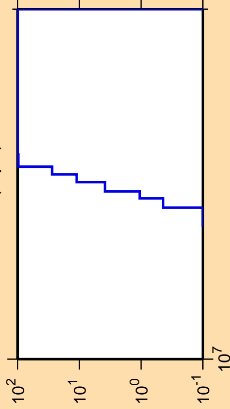
\Delta\sigma/\sigma vs. E for ^{124}\text{Cs}(n,pd)
