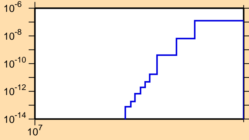
\sigma vs. E for ^{124}\text{Cs}(n,pd)
