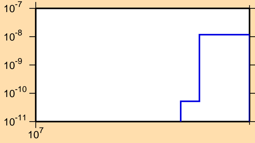
\sigma vs. E for ^{124}\text{Cs}(n,pt)
