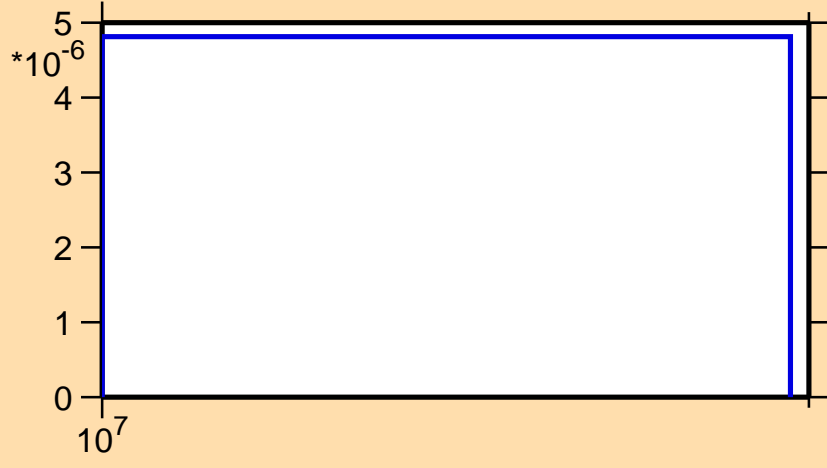
\sigma vs. E for ^{124}\text{Cs}(n,\text{nd})
