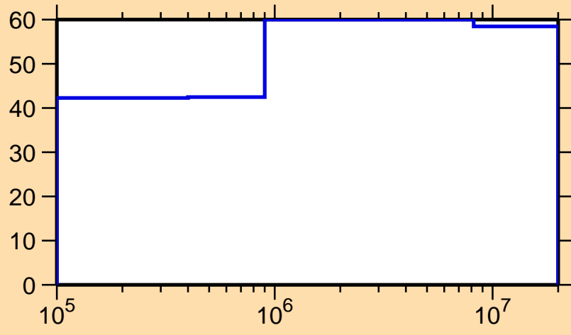
\Delta\sigma/\sigma vs. E for ^{124}\text{Cs}(n,n_1)
