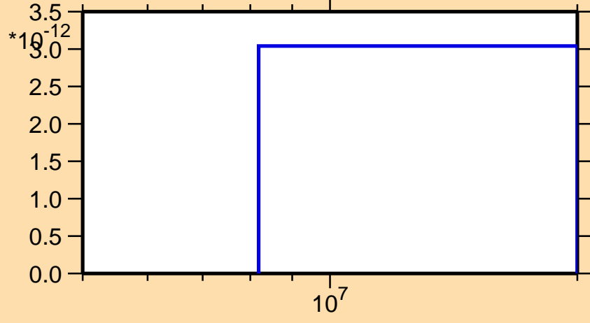
\sigma vs. E for ^{124}\text{Cs}(n,3n)
