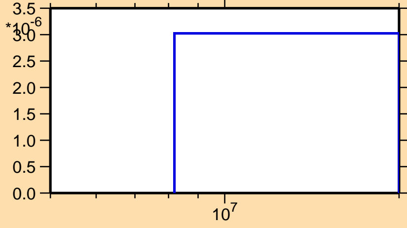
\sigma vs. E for ^{124}\text{Cs}(n,\text{He}3)
