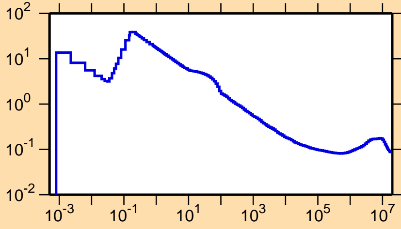
\sigma vs. E for ^{124}\text{Cs}(n,p)
