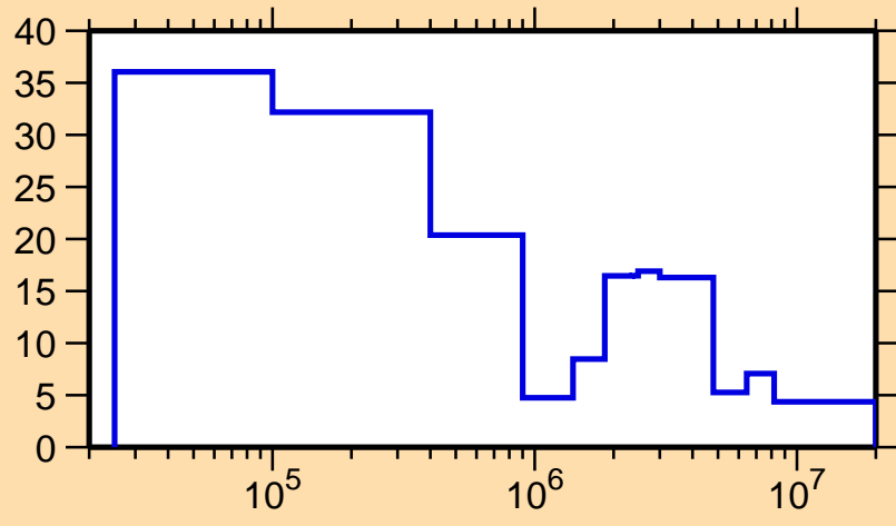
\Delta\sigma/\sigma vs. E for ^{124}\text{Cs}(n, el.)
