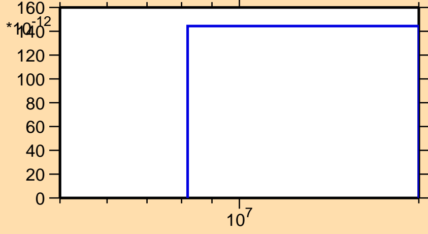
\sigma vs. E for ^{124}\text{Cs}(n,pt)
