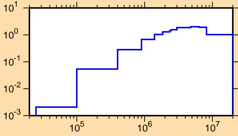
\sigma vs. E for ^{124}\text{Cs}(n,n\text{cont.})
