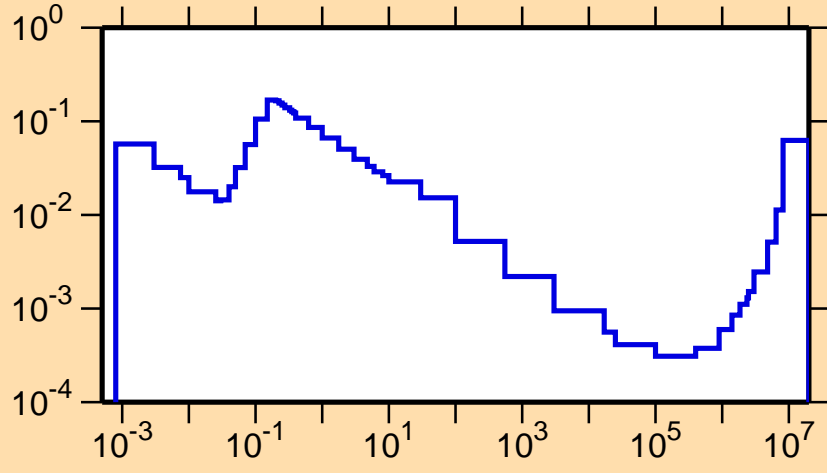
\sigma vs. E for ^{124}\text{Cs}(n,\alpha)
