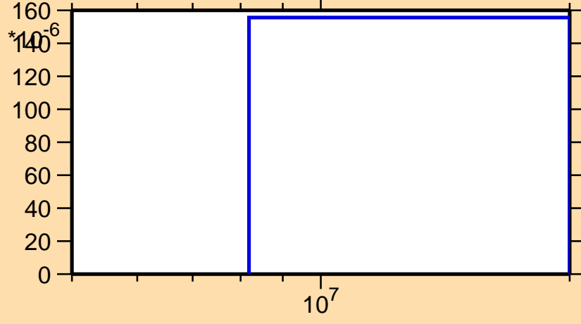
\sigma vs. E for ^{124}\text{Cs}(n,2np)
