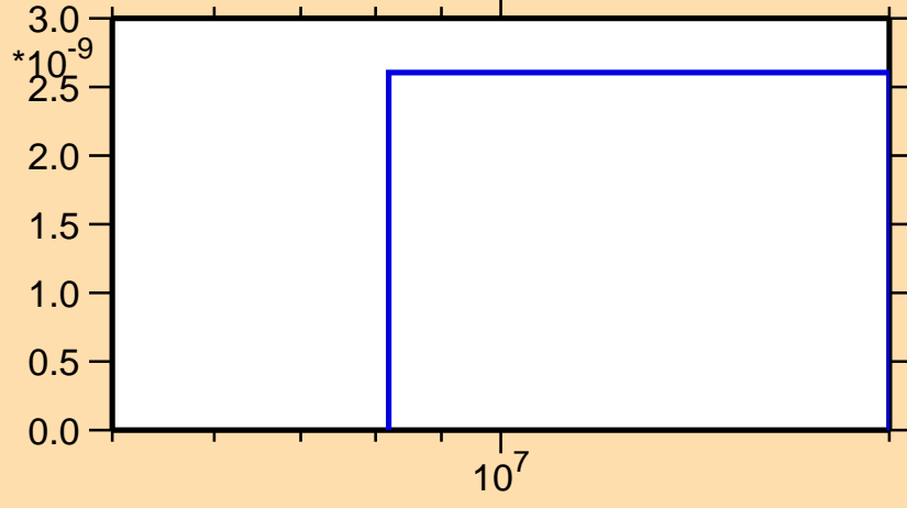
\sigma vs. E for ^{124}\text{Cs} (mt 45)
