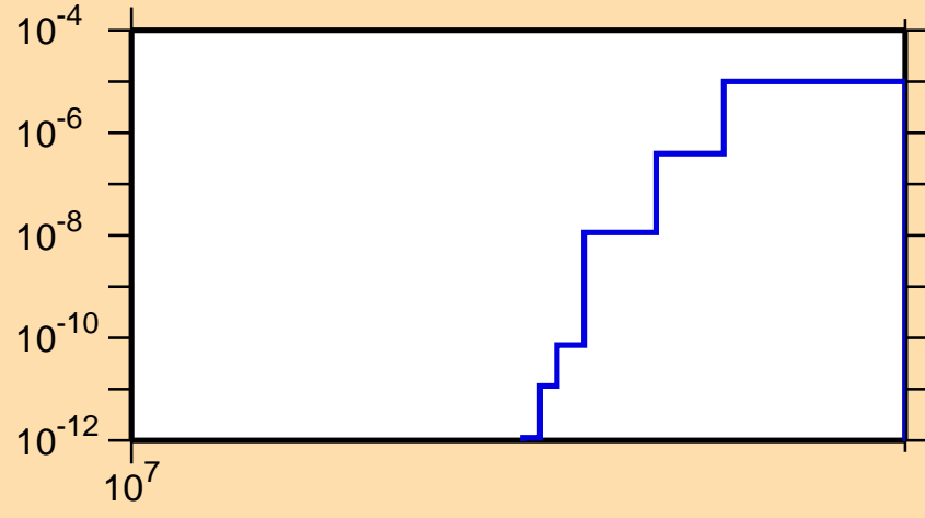
\sigma vs. E for ^{125}\text{Cs}(n,nd)
