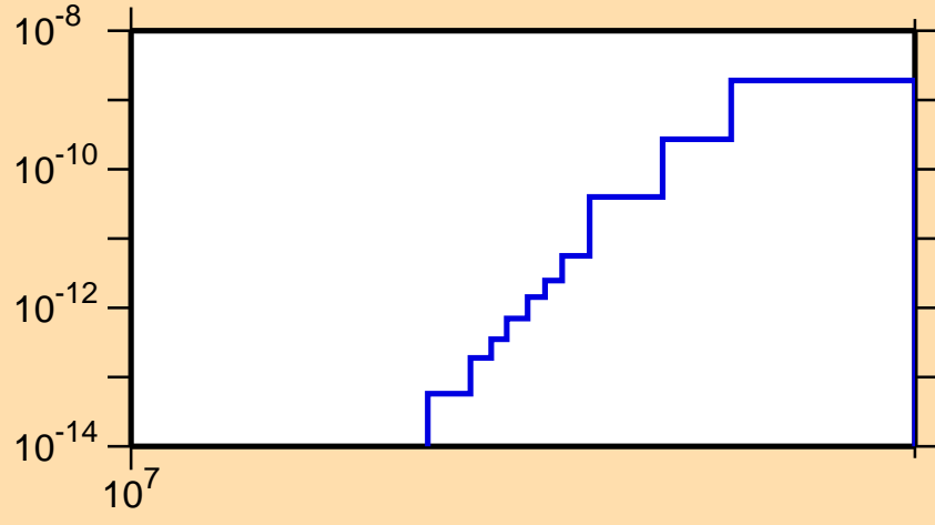
\sigma vs. E for ^{125}\text{Cs}(\text{mt117})
