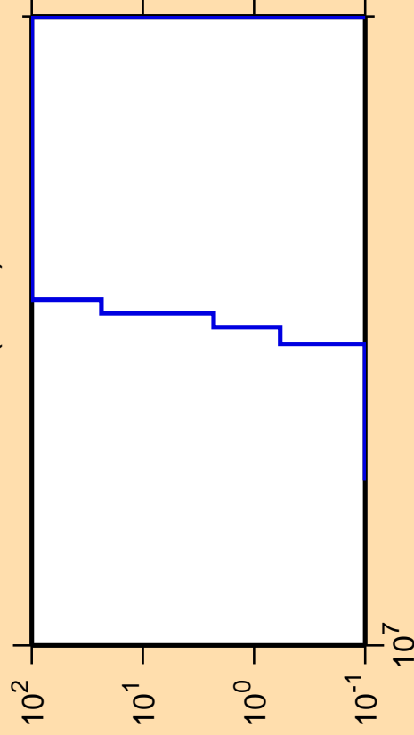
\Delta\sigma/\sigma vs. E for ^{125}\text{Cs}(n,nd)
