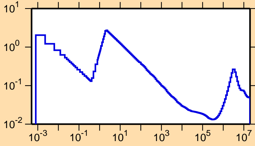
\sigma vs. E for ^{125}\text{Cs}(n,p)
