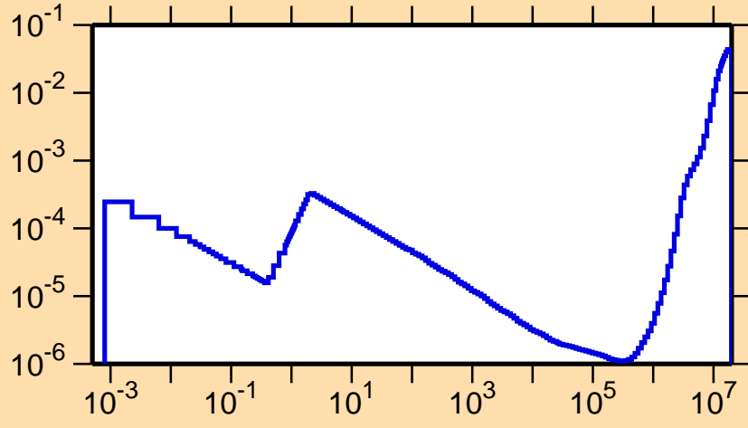
\sigma vs. E for ^{125}\text{Cs}(n,\alpha)
