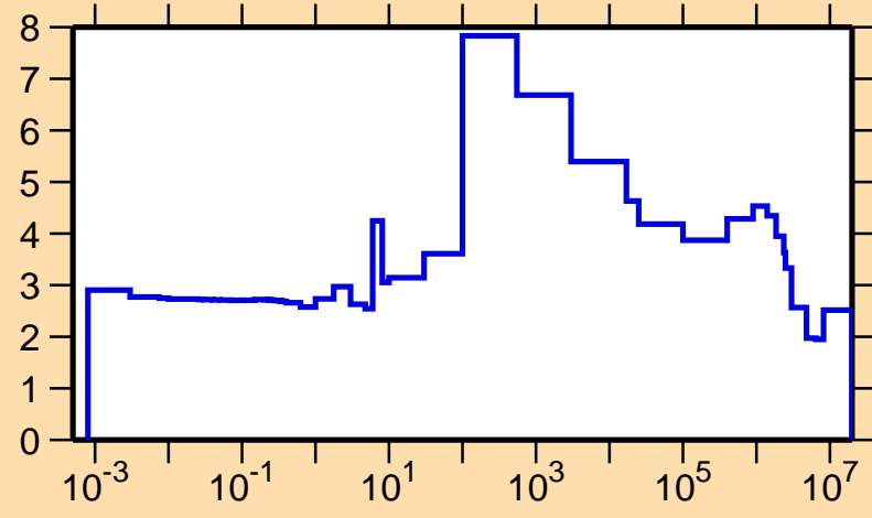
\sigma vs. E for ^{125}\text{Cs}(n,\text{el.})
