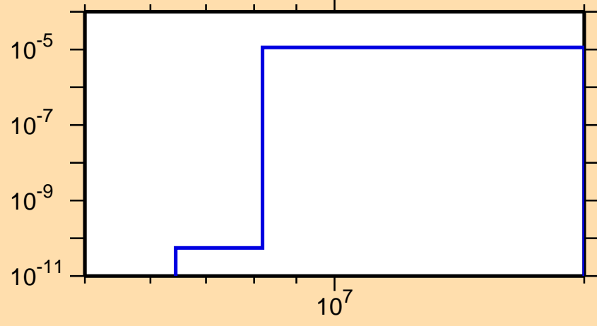
\sigma vs. E for ^{125}\text{Cs}(n,p\alpha)
