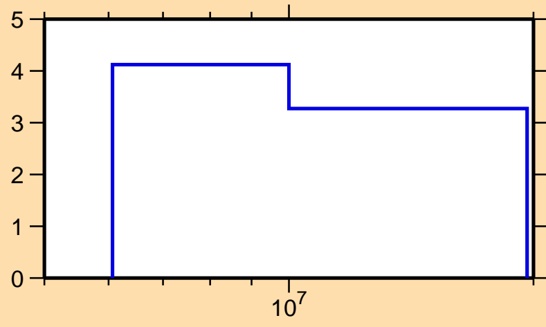
\Delta\sigma/\sigma vs. E for ^{126}\text{Cs}(n,\text{el.})
