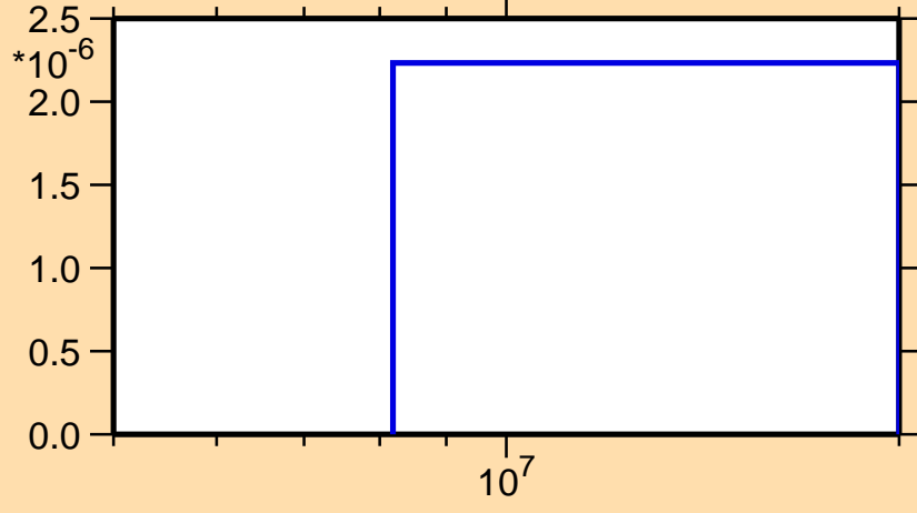
\sigma vs. E for ^{126}\text{Cs}(n,\text{nd})
