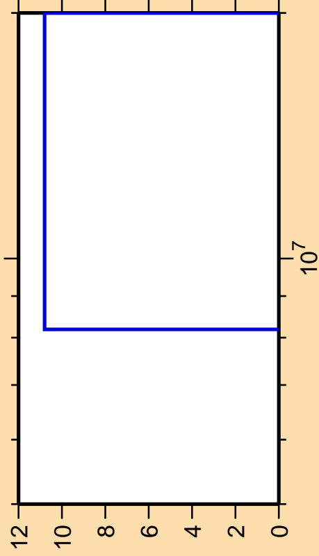
\Delta\sigma/\sigma vs. E for ^{126}\text{Cs}(n,pt)
