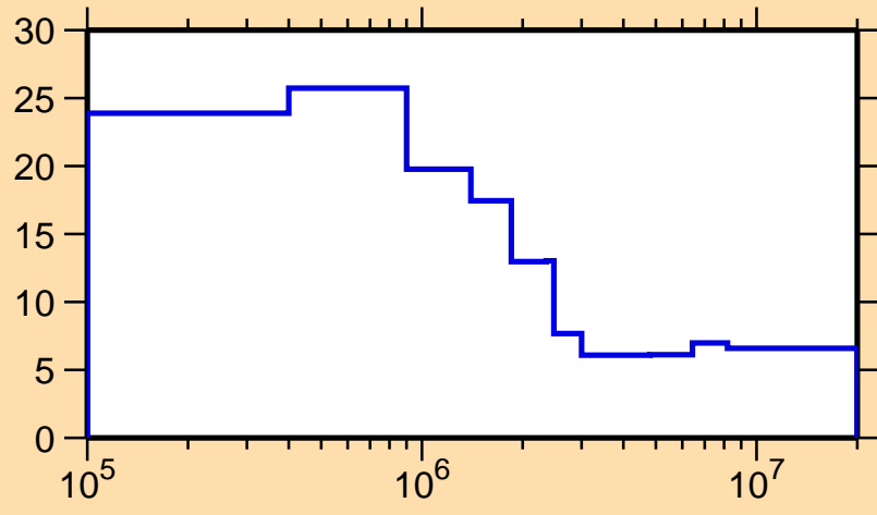
\Delta\sigma/\sigma vs. E for ^{126}\text{Cs}(n,\text{nonel.})
