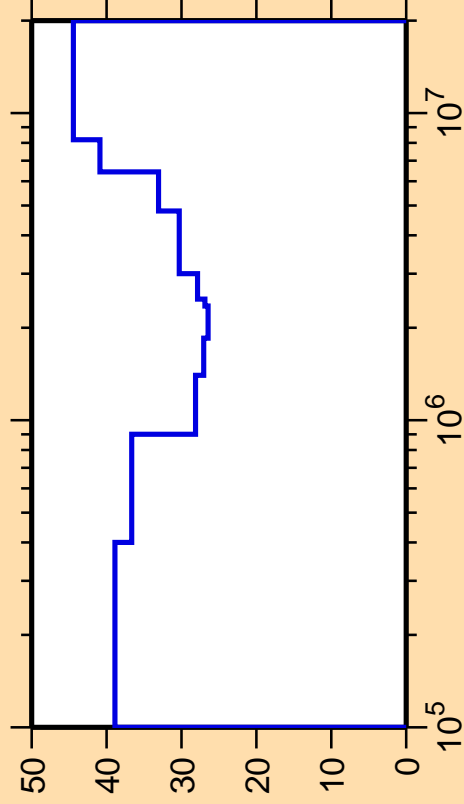
\Delta\sigma/\sigma vs. E for ^{126}\text{Cs}(n,n_4)
