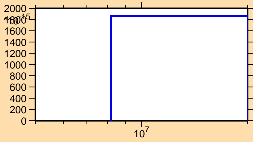
\sigma vs. E for ^{126}\text{Cs}(n,pt)
