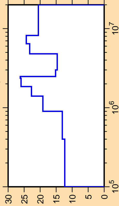
\Delta\sigma/\sigma vs. E for ^{126}\text{Cs}(n,n_3)
