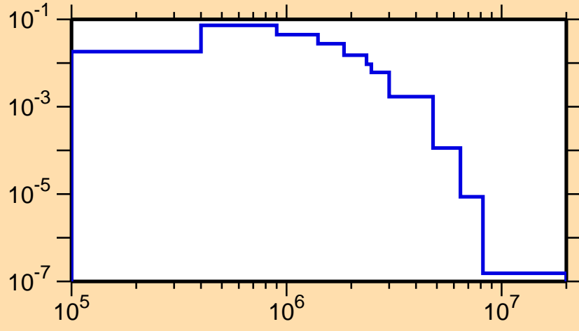
\sigma vs. E for ^{126}\text{Cs}(n,n_4)
