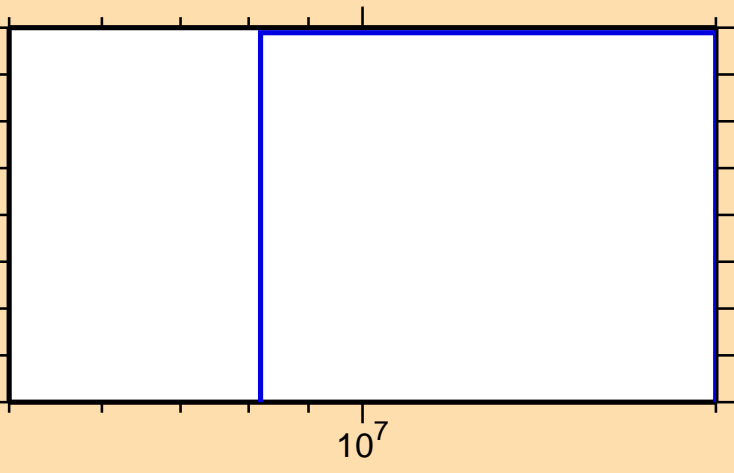
\sigma vs. E for ^{126}\text{Cs}(n,2np)
