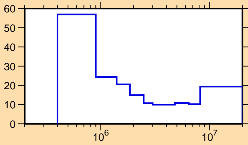
\Delta\sigma/\sigma vs. E for ^{126}\text{Cs}(n,n\text{cont.})
