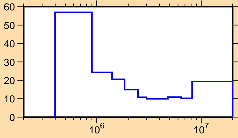
\Delta\sigma/\sigma vs. E for ^{126}\text{Cs}(n,n\text{cont.})
