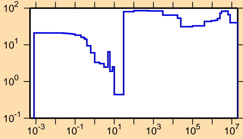
\Delta\sigma/\sigma vs. E for ^{126}\text{Cs}(n,\gamma)
