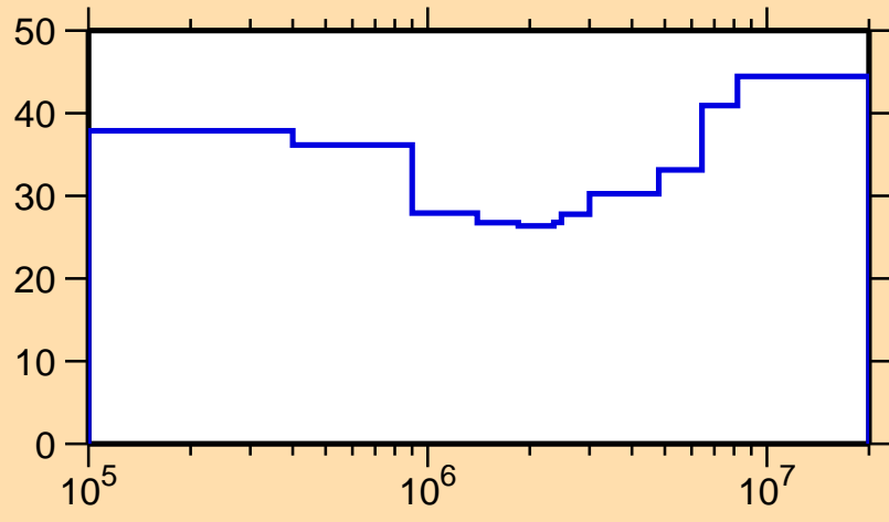
\Delta\sigma/\sigma vs. E for ^{126}\text{Cs}(n,n_1)
