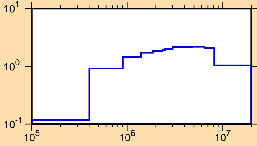
\sigma vs. E for ^{126}\text{Cs}(n,\text{inel.})
