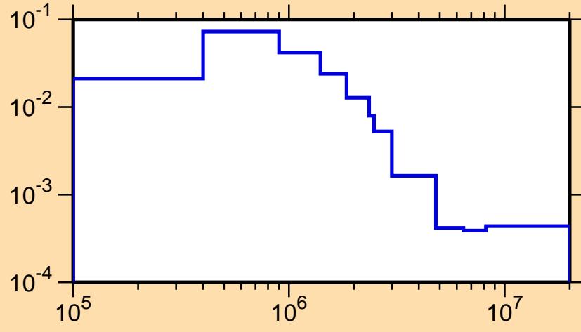
\sigma vs. E for ^{126}\text{Cs}(n,n_3)
