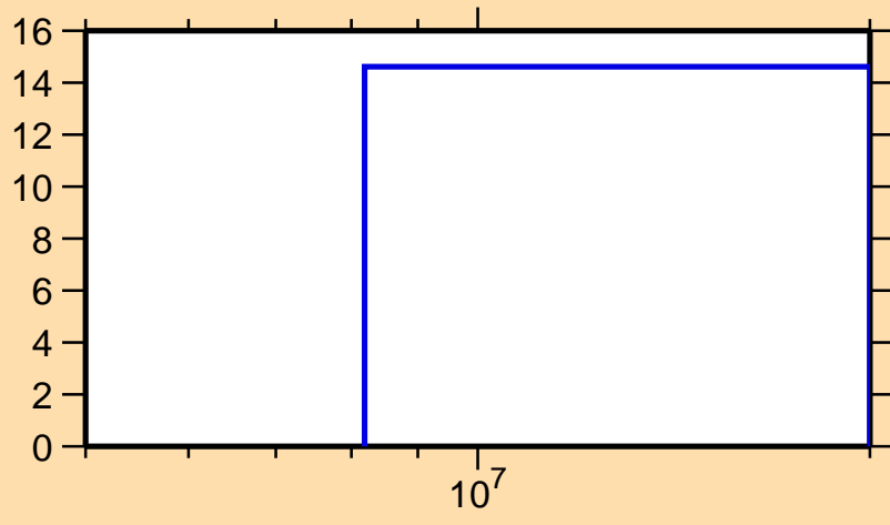
\Delta\sigma/\sigma vs. E for ^{126}\text{Cs}(n,2n)
