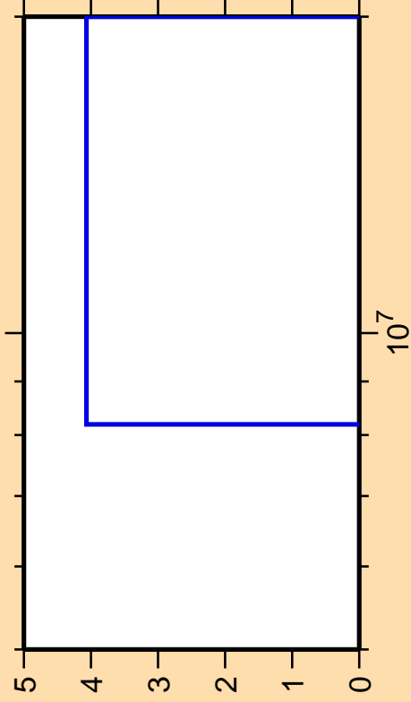
\Delta\sigma/\sigma vs. E for ^{127}\text{Cs}(n,\text{pd})
