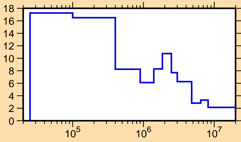
\Delta\sigma/\sigma vs. E for ^{127}\text{Cs}(n,\text{tot.})
