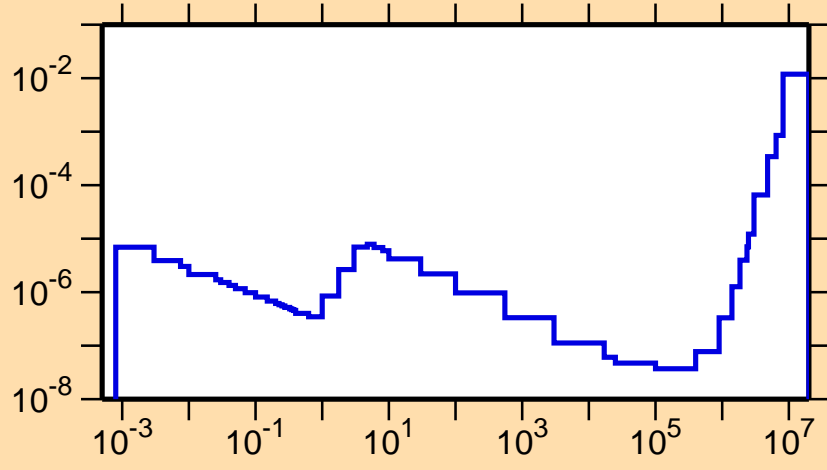
\sigma vs. E for ^{127}\text{Cs}(n,\alpha)
