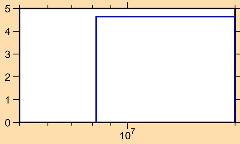
\Delta\sigma/\sigma vs. E for ^{127}\text{Cs}(n,\text{nonel.})
