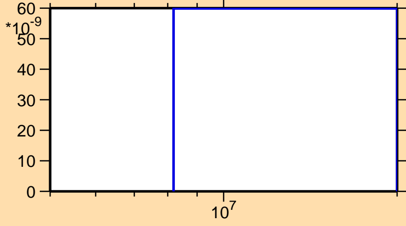
\sigma vs. E for ^{127}\text{Cs}(n,\text{nd})
