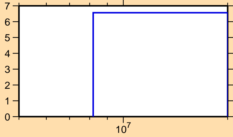
\Delta\sigma/\sigma vs. E for ^{127}\text{Cs}(n,2n)
