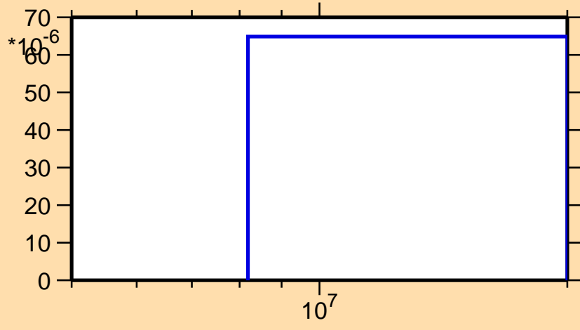
\sigma vs. E for ^{127}\text{Cs}(n,t)
