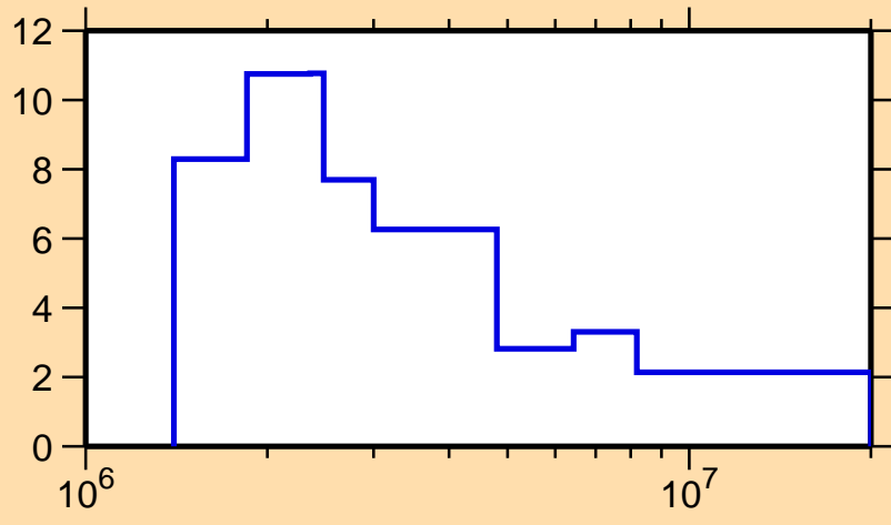
\Delta\sigma/\sigma vs. E for ^{127}\text{Cs}(n, tot.)
