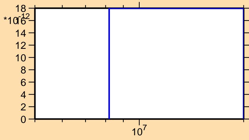
\sigma vs. E for ^{127}\text{Cs}(n,2n\alpha)
