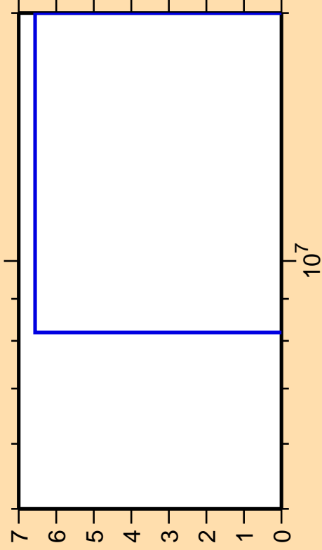
\Delta\sigma/\sigma vs. E for ^{127}\text{Cs}(n,2n)
