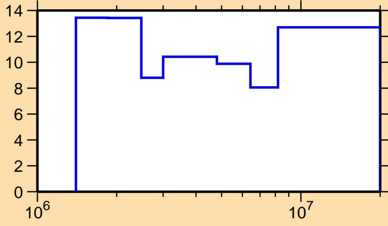
\Delta\sigma/\sigma vs. E for ^{127}\text{Cs}(n,n\text{cont.})
