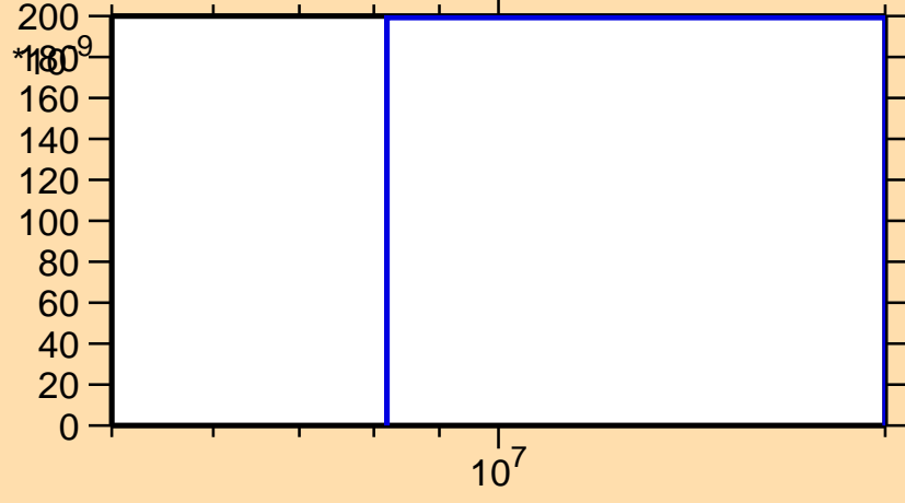
\sigma vs. E for ^{127}\text{Cs}(n,p\alpha)
