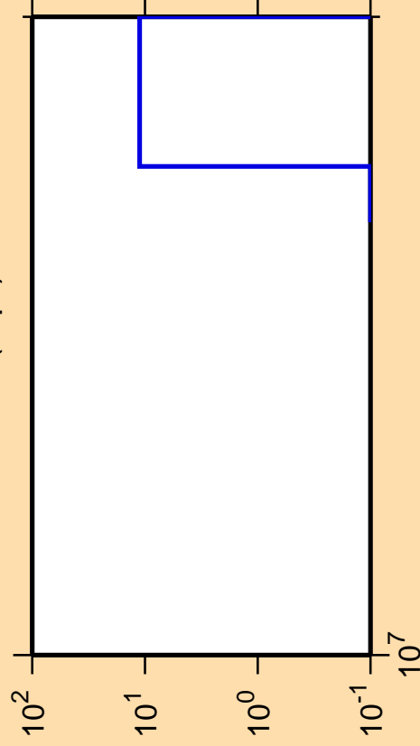
\Delta\sigma/\sigma vs. E for ^{128}\text{Cs}(n,pt)
