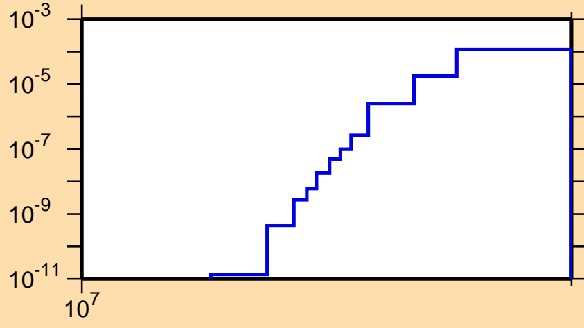
\sigma vs. E for ^{128}\text{Cs}(n,nd)
