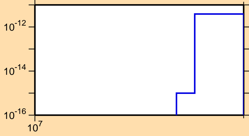
\sigma vs. E for ^{128}\text{Cs}(n,pt)
