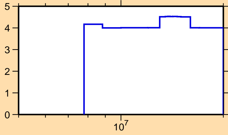
\Delta\sigma/\sigma vs. E for ^{128}\text{Cs}(n,\text{nonel.})
