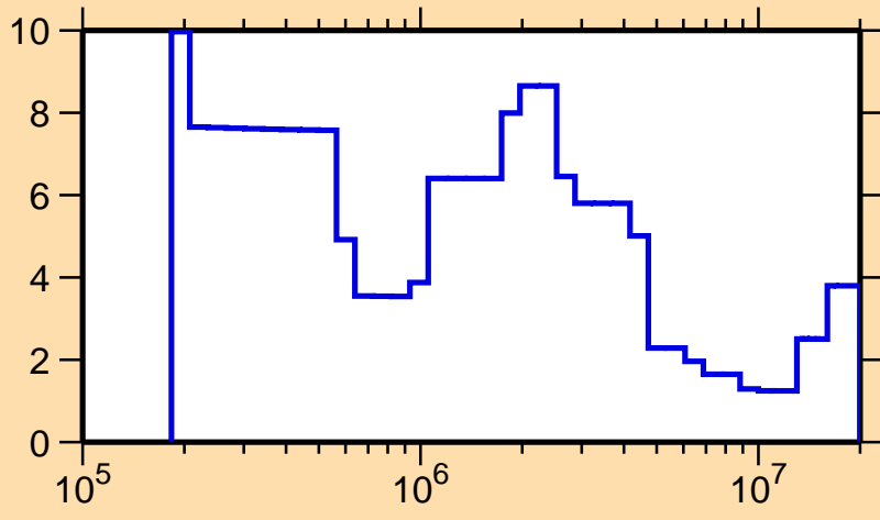
\Delta\sigma/\sigma vs. E for ^{128}\text{Cs}(n,\text{tot.})
