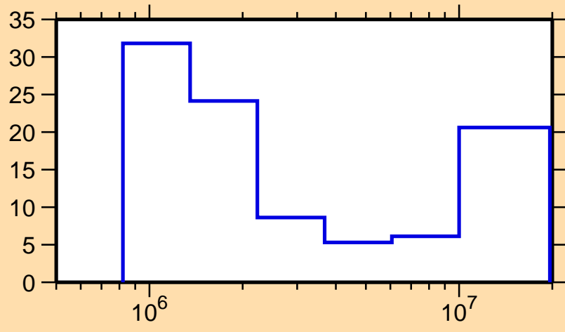
\Delta\sigma/\sigma vs. E for ^{128}\text{Cs}(n,n\text{cont.})
