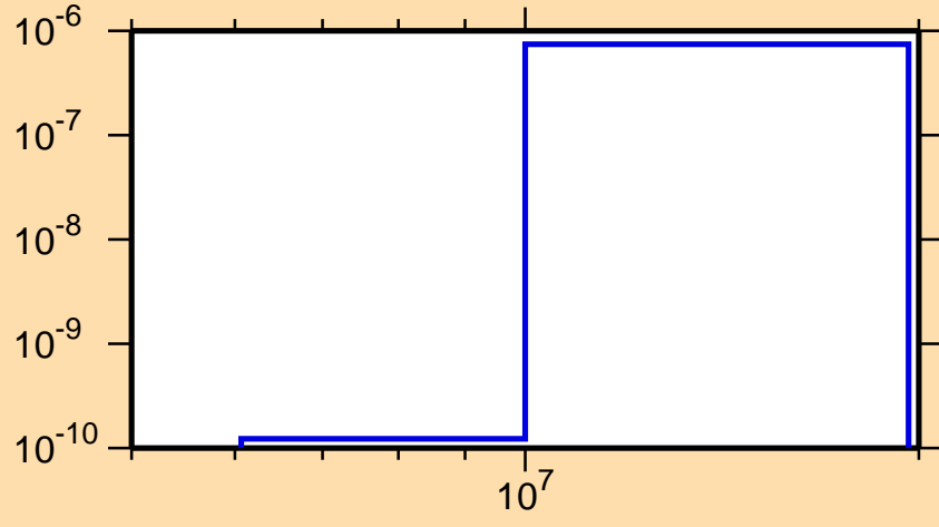
\sigma vs. E for ^{128}\text{Cs}(n,p\alpha)
