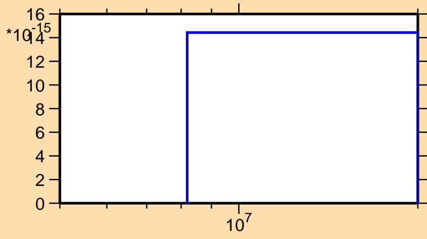
\sigma vs. E for ^{128}\text{Cs} (mt 34)
