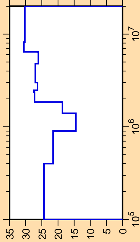
\Delta\sigma/\sigma vs. E for ^{128}\text{Cs}(n,n_4)
