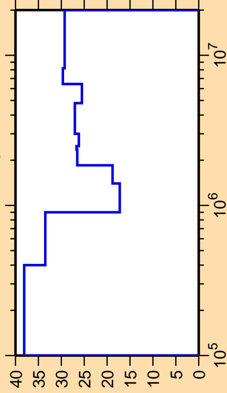
\Delta\sigma/\sigma vs. E for ^{128}\text{Cs}(n,n_3)
