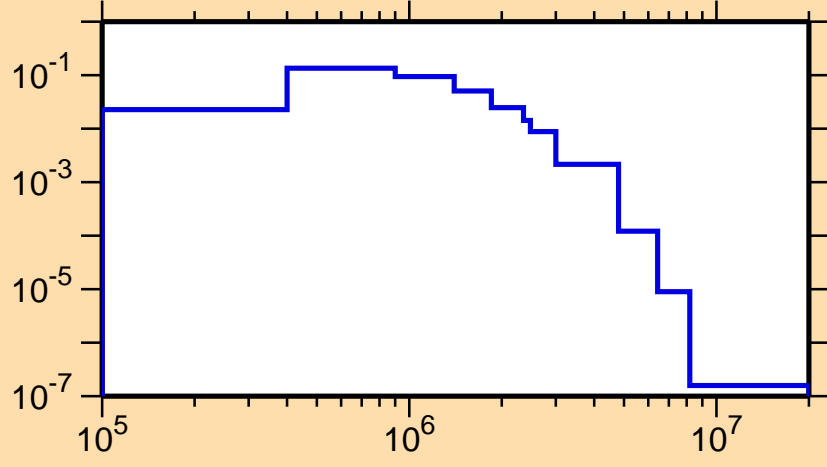
\sigma vs. E for ^{128}\text{Cs}(n,n_4)
