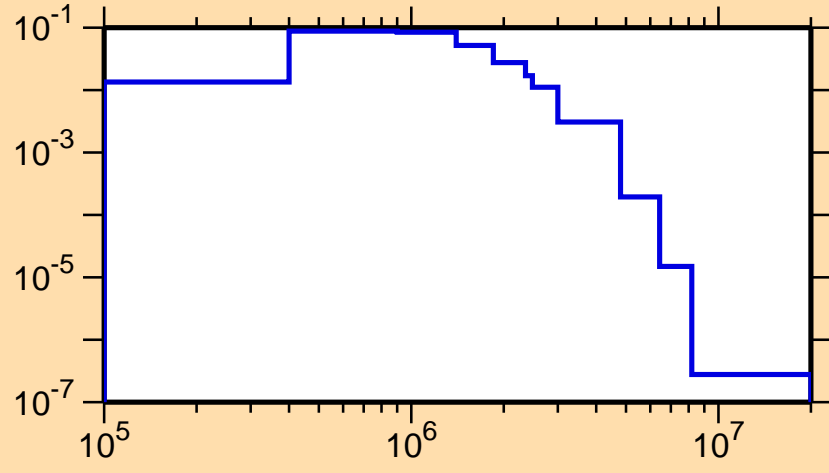
\sigma vs. E for ^{128}\text{Cs}(n,n_3)
