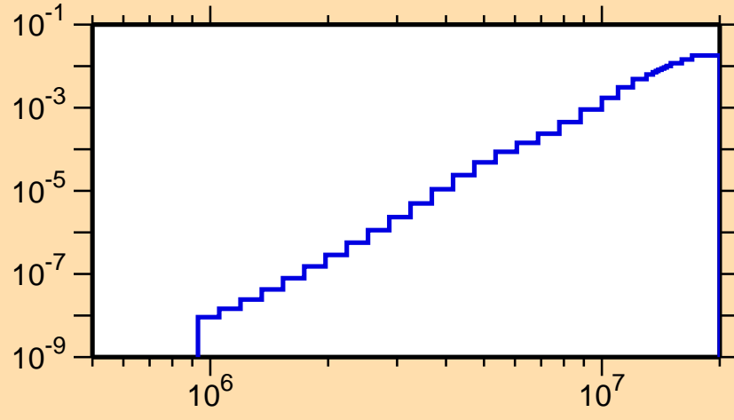
\sigma vs. E for ^{129}\text{Cs}(n,\alpha)
