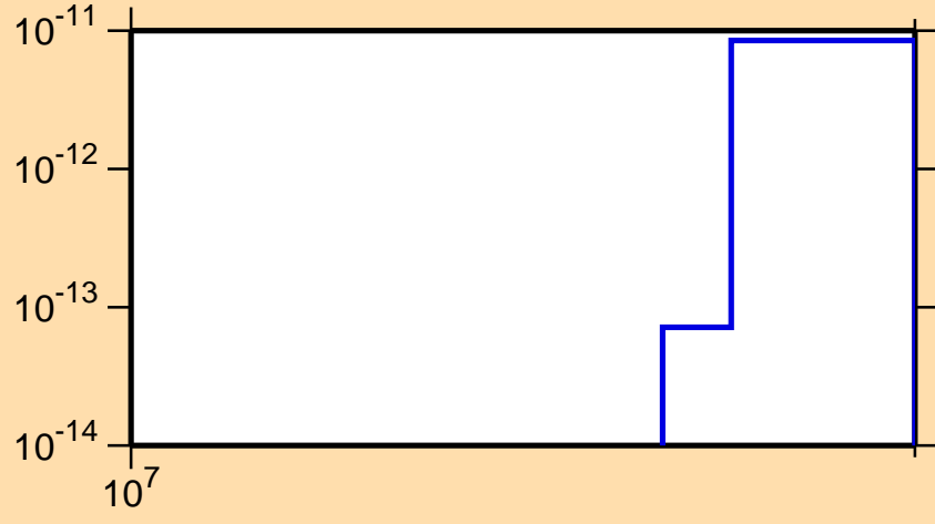
\sigma vs. E for ^{129}\text{Cs} (mt 45)
