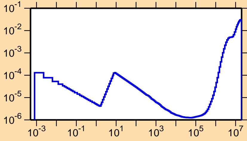
\sigma vs. E for ^{129}\text{Cs}(n,p)
