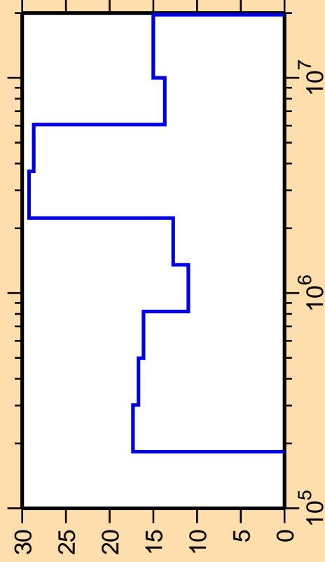
\Delta\sigma/\sigma vs. E for ^{129}\text{Cs}(n,n_4)
