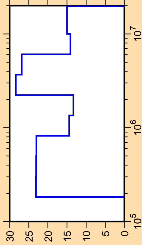
\Delta\sigma/\sigma vs. E for ^{129}\text{Cs}(n,n_3)
