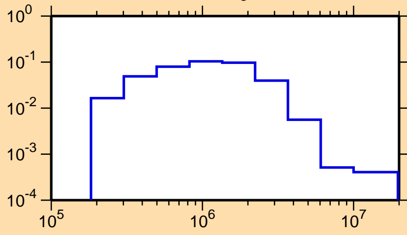
\sigma vs. E for ^{129}\text{Cs}(n,n_3)
