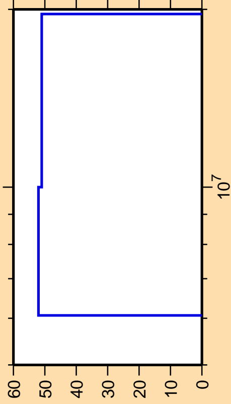
\Delta\sigma/\sigma vs. E for ^{129}\text{Cs}(n,n\alpha)
