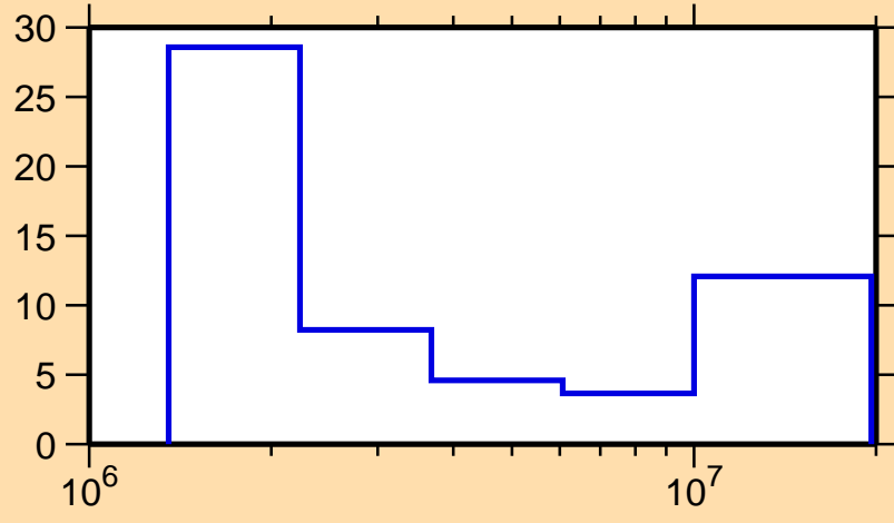
\Delta\sigma/\sigma vs. E for ^{129}\text{Cs}(n,n\text{cont.})
