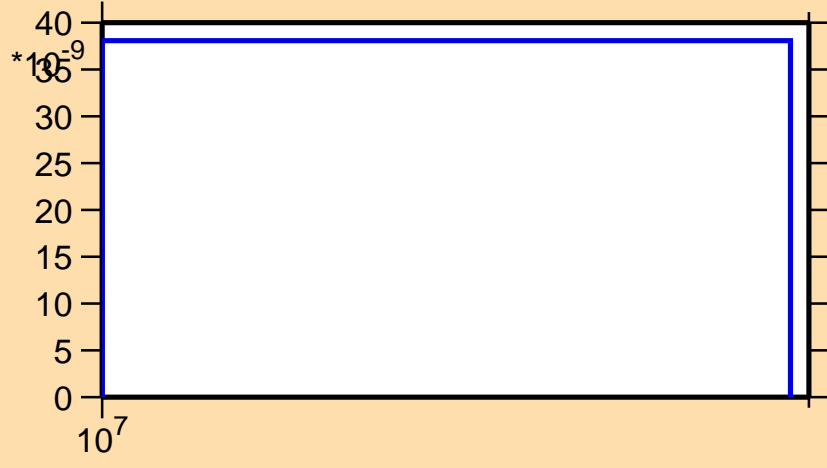
\sigma vs. E for ^{129}\text{Cs}(n,2np)
