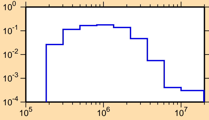
\sigma vs. E for ^{129}\text{Cs}(n,n_4)
