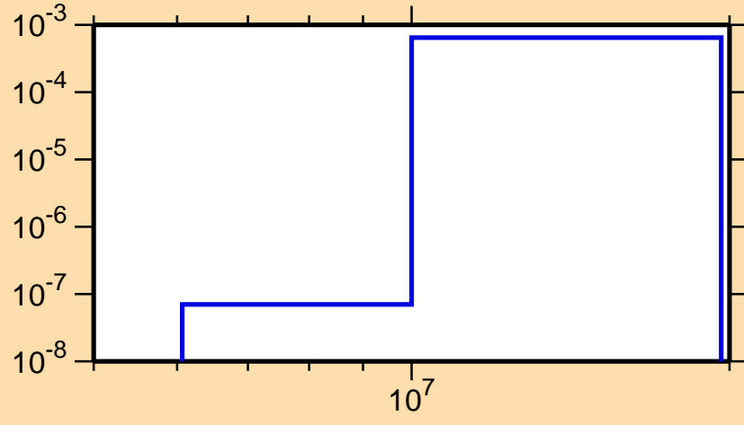
\sigma vs. E for ^{129}\text{Cs}(n,n\alpha)
