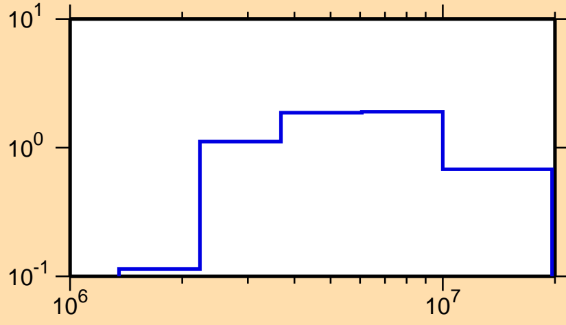
\sigma vs. E for ^{129}\text{Cs}(n,n\text{cont.})
