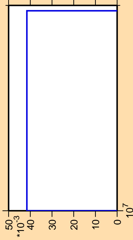
\Delta\sigma/\sigma vs. E for ^{129}\text{Cs} (mt 45)
