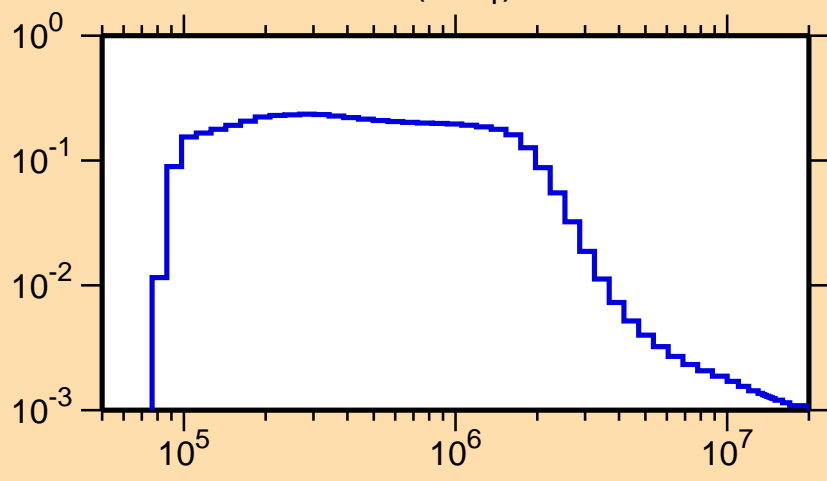
\sigma vs. E for ^{130}\text{Cs}(n,n_1)
