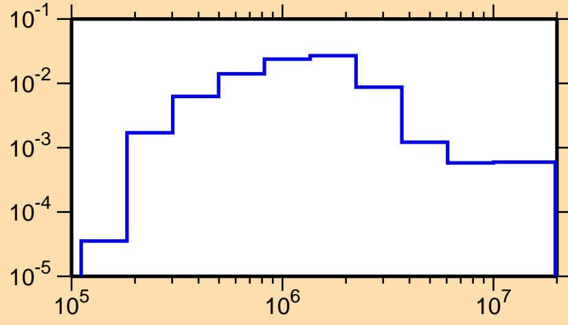
\sigma vs. E for ^{130}\text{Cs}(n,n_4)
