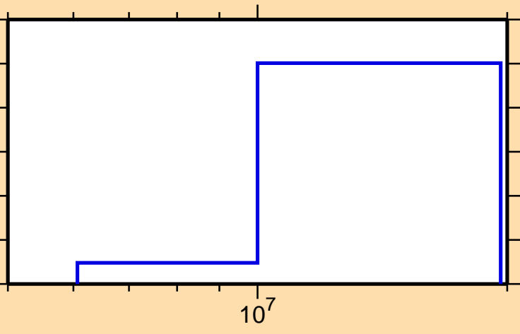
\sigma vs. E for ^{130}\text{Cs}(n,p\alpha)
