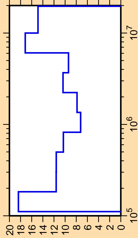
\Delta\sigma/\sigma vs. E for ^{130}\text{Cs}(n,n_4)
