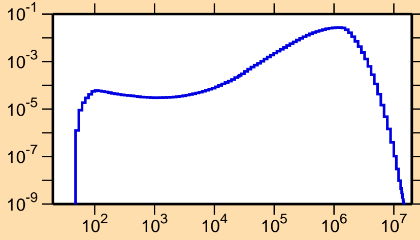
\sigma vs. E for ^{130}\text{Cs}(n,n_3)
