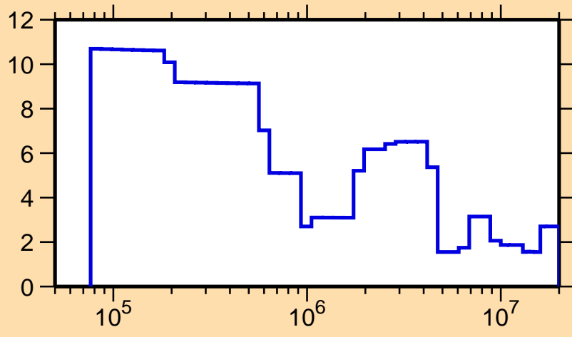
\Delta\sigma/\sigma vs. E for ^{131}\text{Cs}(n,\text{el.})
