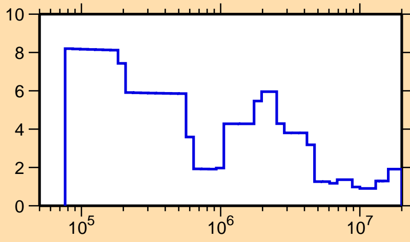
\Delta\sigma/\sigma vs. E for ^{131}\text{Cs}(n,\text{tot.})
