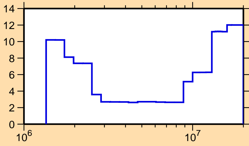
\Delta\sigma/\sigma vs. E for ^{131}\text{Cs}(n,\text{inel.})
