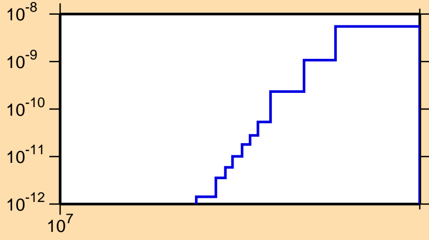
\sigma vs. E for ^{131}\text{Cs}(n,p\alpha)
