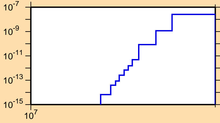
\sigma vs. E for ^{131}\text{Cs}(n,\text{He}3)
