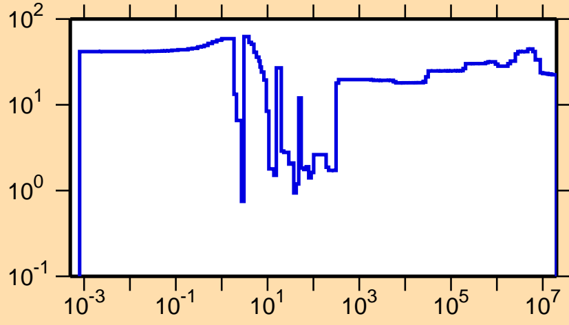
\Delta\sigma/\sigma vs. E for ^{131}\text{Cs}(n,\gamma)
