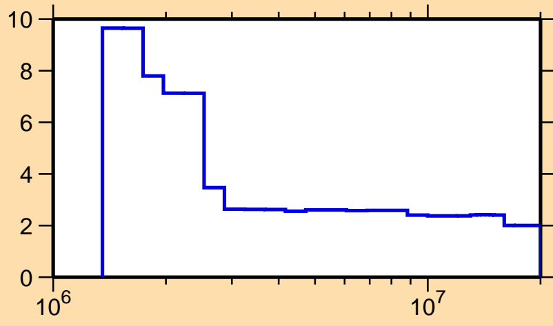
\Delta\sigma/\sigma vs. E for ^{131}\text{Cs}(n,\text{nonel.})
